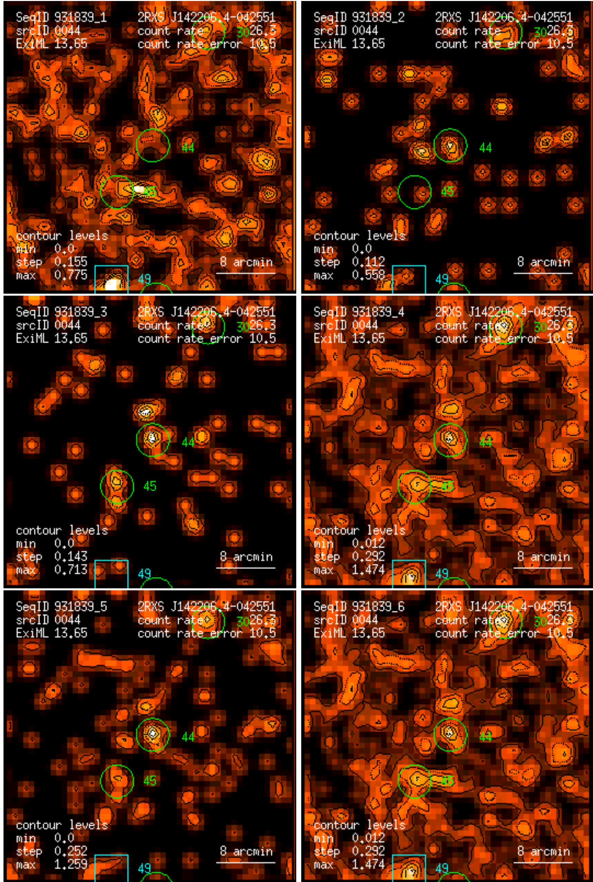
Figure 44: RASS 931839: detection 0044: band rate images, Gaussian filter: (1) PSPC channels 11 – 41, (2) 52 – 90, (3) 91 – 201, (4) 11 – 235, (5) 52 – 201, (6) 11 – 201. Broad band rates in counts/ks. Band rate contour levels in counts/ks/arcmin 2 .
