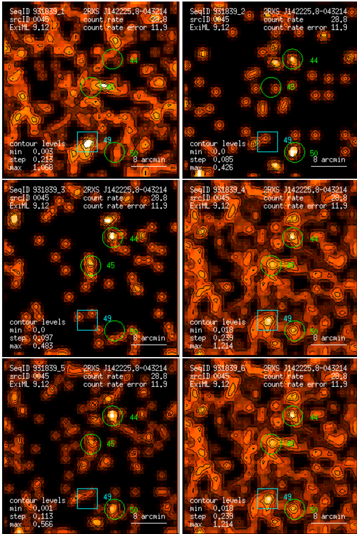
Figure 45: RASS 931839: detection 0045: band rate images, Gaussian filter: (1) PSPC channels 11 – 41, (2) 52 – 90, (3) 91 – 201, (4) 11 – 235, (5) 52 – 201, (6) 11 – 201. Broad band rates in counts/ks. Band rate contour levels in counts/ks/arcmin 2 .
