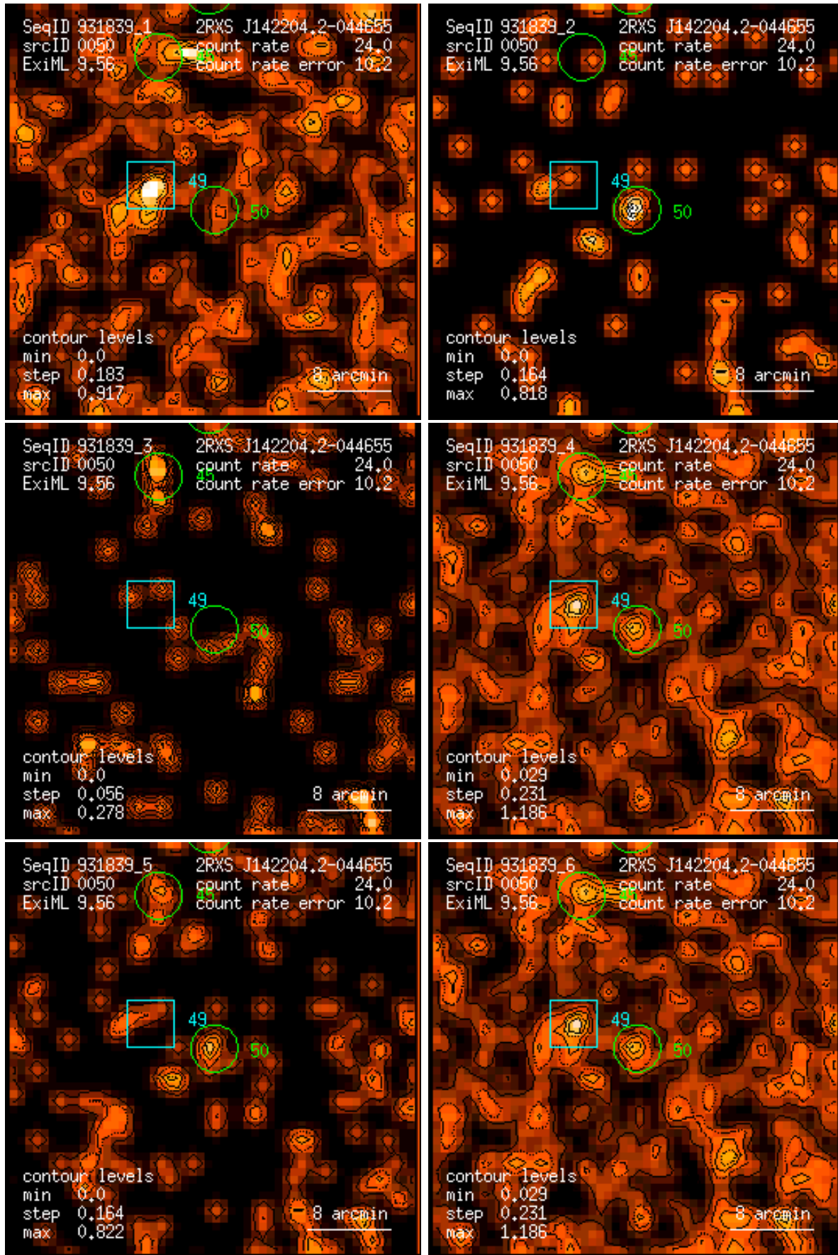
Figure 50: RASS 931839: detection 0050: band rate images, Gaussian filter: (1) PSPC channels 11 – 41, (2) 52 – 90, (3) 91 – 201, (4) 11 – 235, (5) 52 – 201, (6) 11 – 201. Broad band rates in counts/ks. Band rate contour levels in counts/ks/arcmin 2 .
