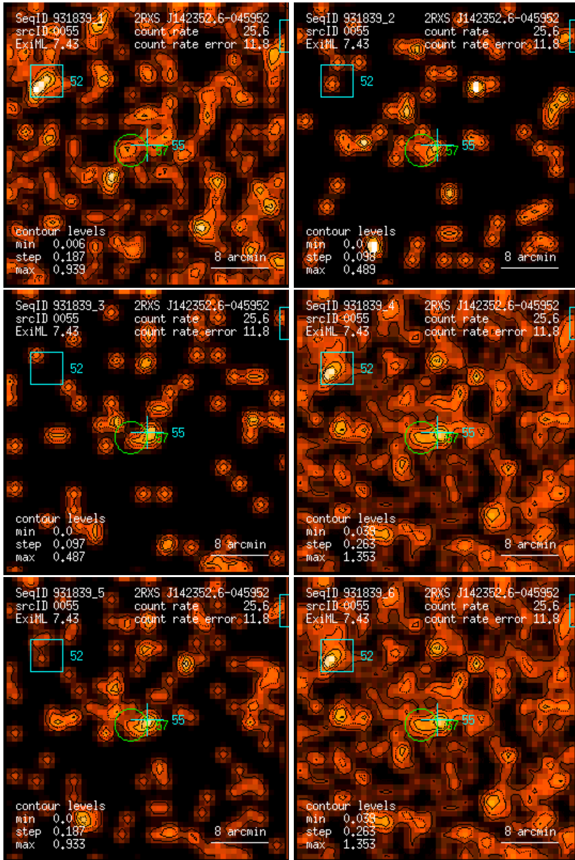
Figure 55: RASS 931839: detection 0055: band rate images, Gaussian filter: (1) PSPC channels 11 – 41, (2) 52 – 90, (3) 91 – 201, (4) 11 – 235, (5) 52 – 201, (6) 11 – 201. Broad band rates in counts/ks. Band rate contour levels in counts/ks/arcmin 2 .
