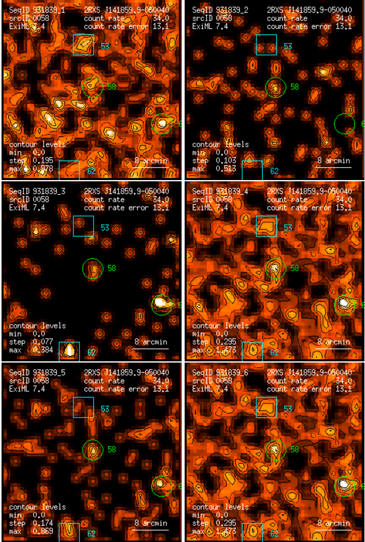
Figure 58: RASS 931839: detection 0058: band rate images, Gaussian filter: (1) PSPC channels 11 – 41, (2) 52 – 90, (3) 91 – 201, (4) 11 – 235, (5) 52 – 201, (6) 11 – 201. Broad band rates in counts/ks. Band rate contour levels in counts/ks/arcmin 2 .
