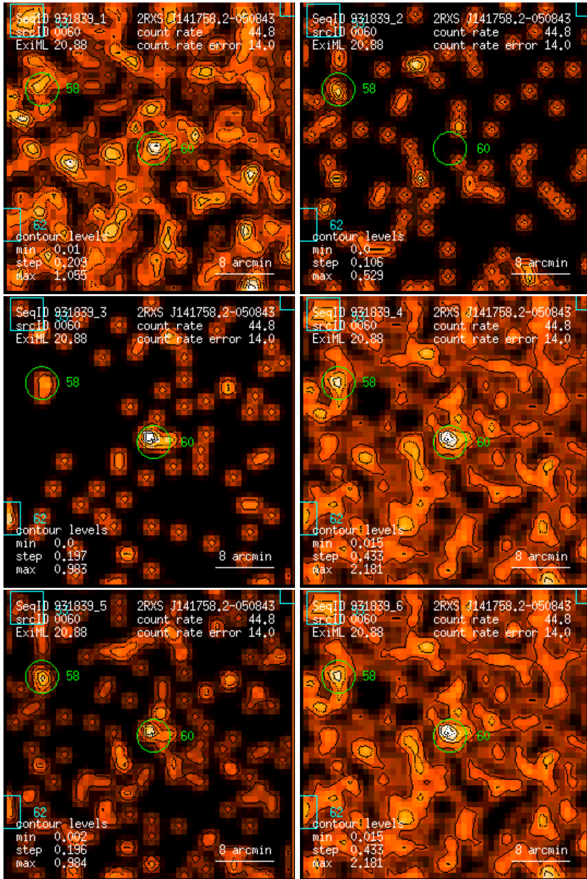
Figure 60: RASS 931839: detection 0060: band rate images, Gaussian filter: (1) PSPC channels 11 – 41, (2) 52 – 90, (3) 91 – 201, (4) 11 – 235, (5) 52 – 201, (6) 11 – 201. Broad band rates in counts/ks. Band rate contour levels in counts/ks/arcmin 2 .
