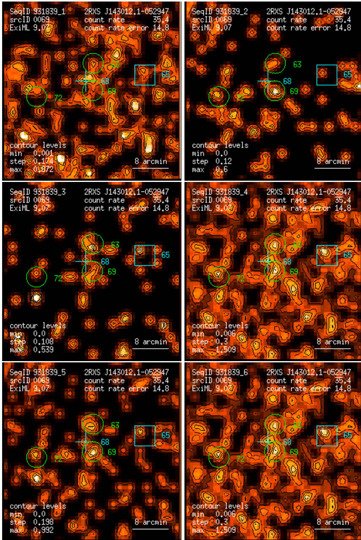
Figure 69: RASS 931839: detection 0069: band rate images, Gaussian filter: (1) PSPC channels 11 – 41, (2) 52 – 90, (3) 91 – 201, (4) 11 – 235, (5) 52 – 201, (6) 11 – 201. Broad band rates in counts/ks. Band rate contour levels in counts/ks/arcmin 2 .
