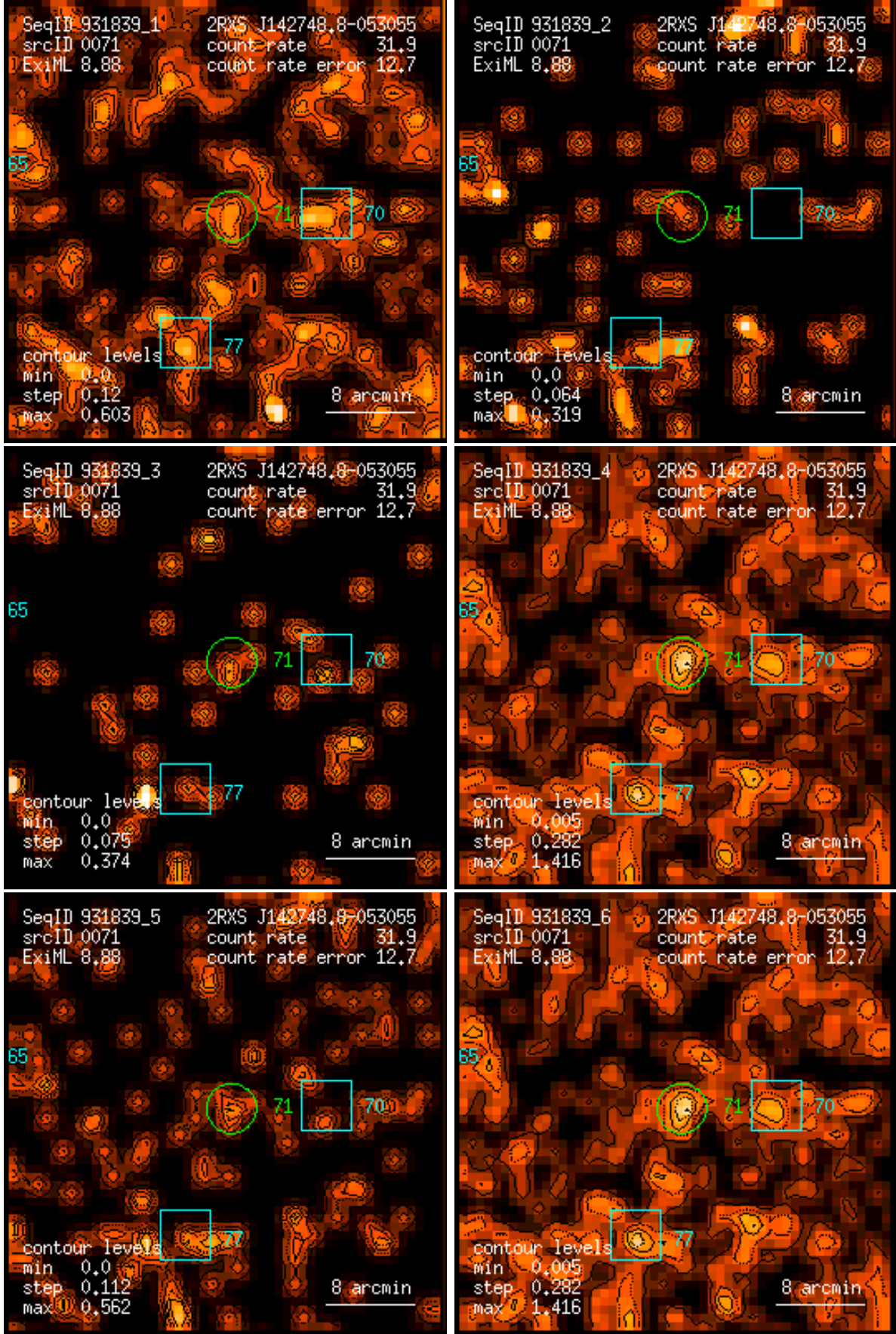
Figure 71: RASS 931839: detection 0071: band rate images, Gaussian filter: (1) PSPC channels 11 – 41, (2) 52 – 90, (3) 91 – 201, (4) 11 – 235, (5) 52 – 201, (6) 11 – 201. Broad band rates in counts/ks. Band rate contour levels in counts/ks/arcmin 2 .
