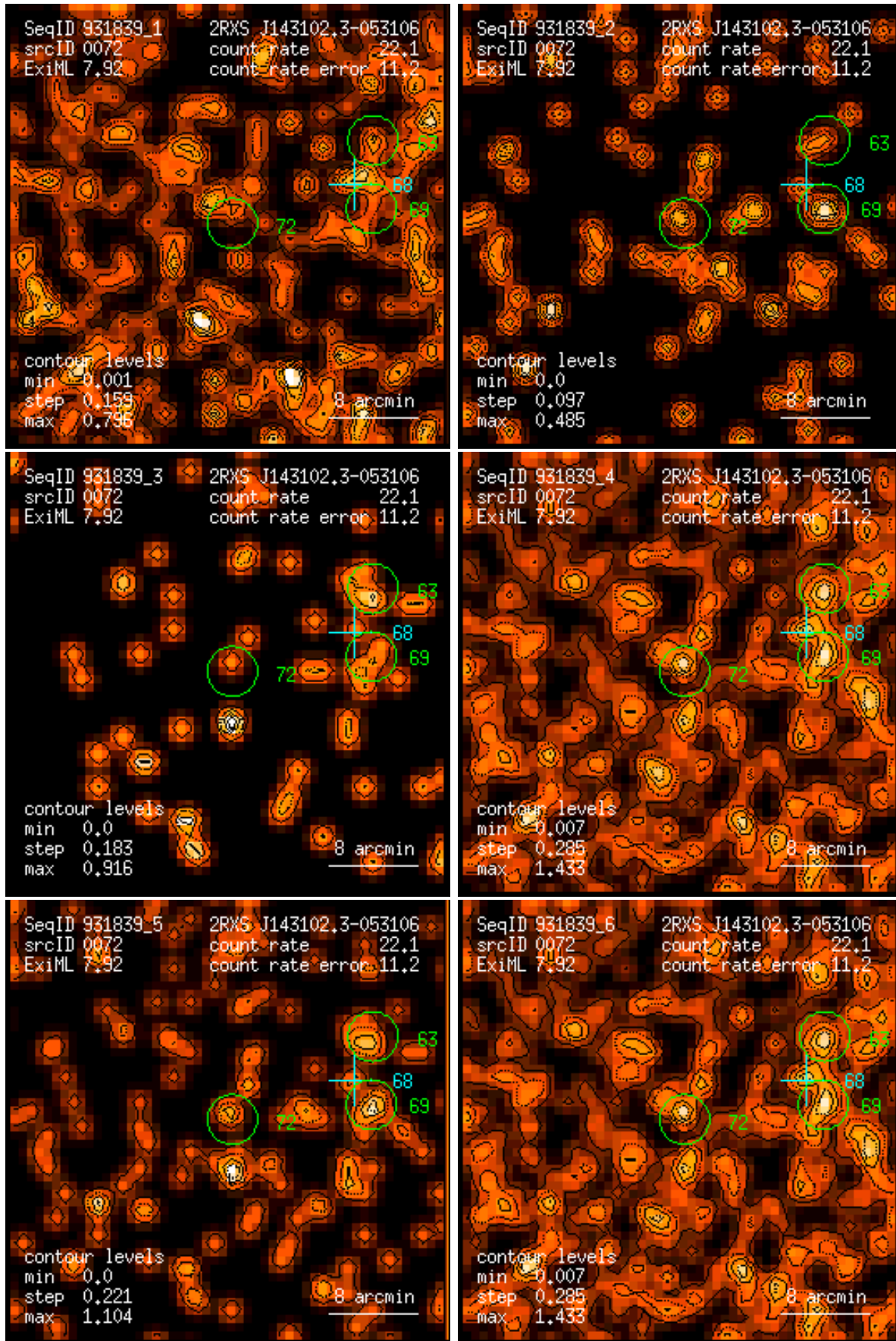
Figure 72: RASS 931839: detection 0072: band rate images, Gaussian filter: (1) PSPC channels 11 – 41, (2) 52 – 90, (3) 91 – 201, (4) 11 – 235, (5) 52 – 201, (6) 11 – 201. Broad band rates in counts/ks. Band rate contour levels in counts/ks/arcmin 2 .
