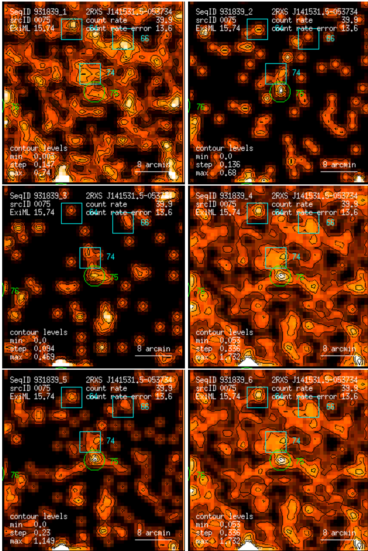
Figure 75: RASS 931839: detection 0075: band rate images, Gaussian filter: (1) PSPC channels 11 – 41, (2) 52 – 90, (3) 91 – 201, (4) 11 – 235, (5) 52 – 201, (6) 11 – 201. Broad band rates in counts/ks. Band rate contour levels in counts/ks/arcmin 2 .
