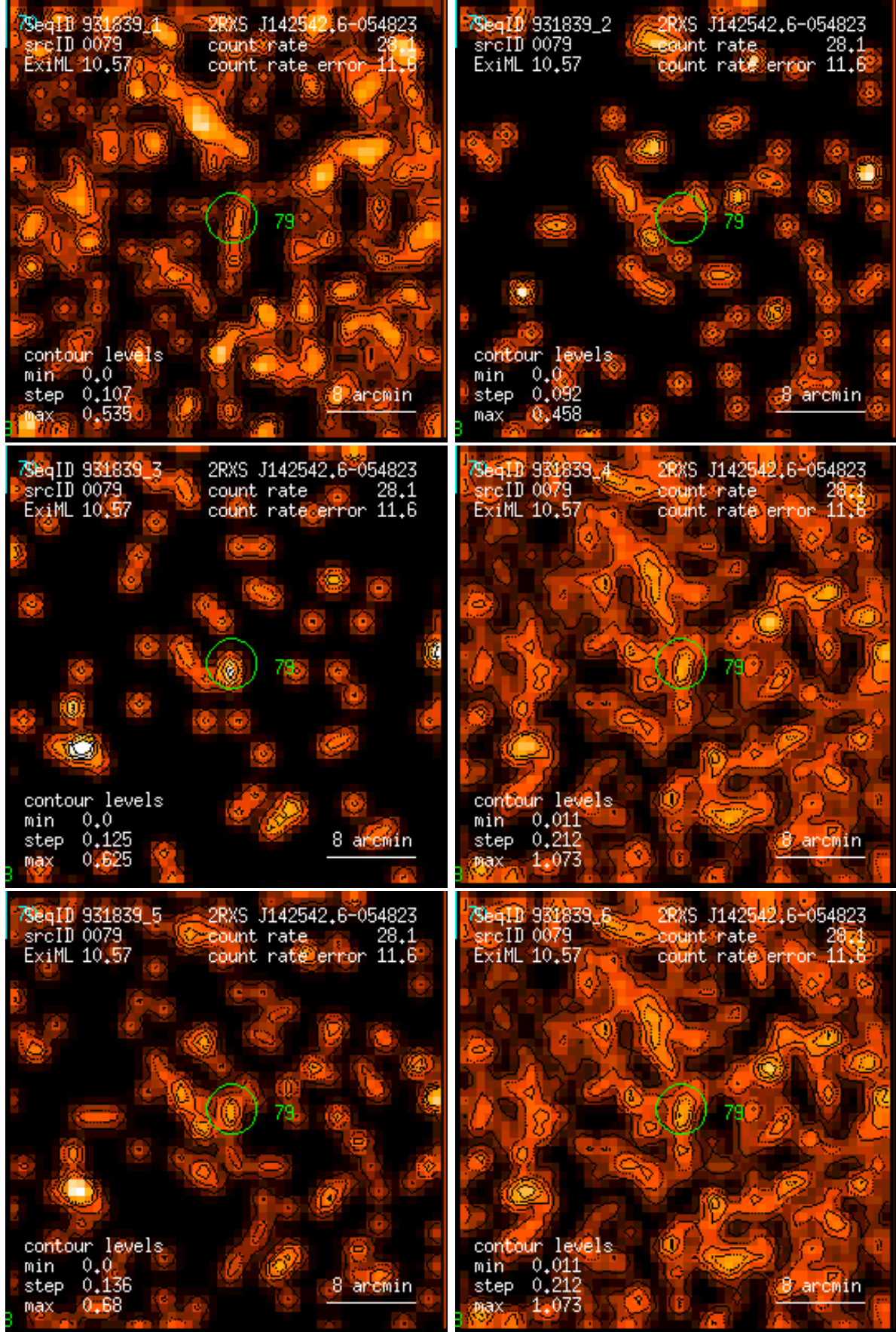
Figure 79: RASS 931839: detection 0079: band rate images, Gaussian filter: (1) PSPC channels 11 – 41, (2) 52 – 90, (3) 91 – 201, (4) 11 – 235, (5) 52 – 201, (6) 11 – 201. Broad band rates in counts/ks. Band rate contour levels in counts/ks/arcmin 2 .
