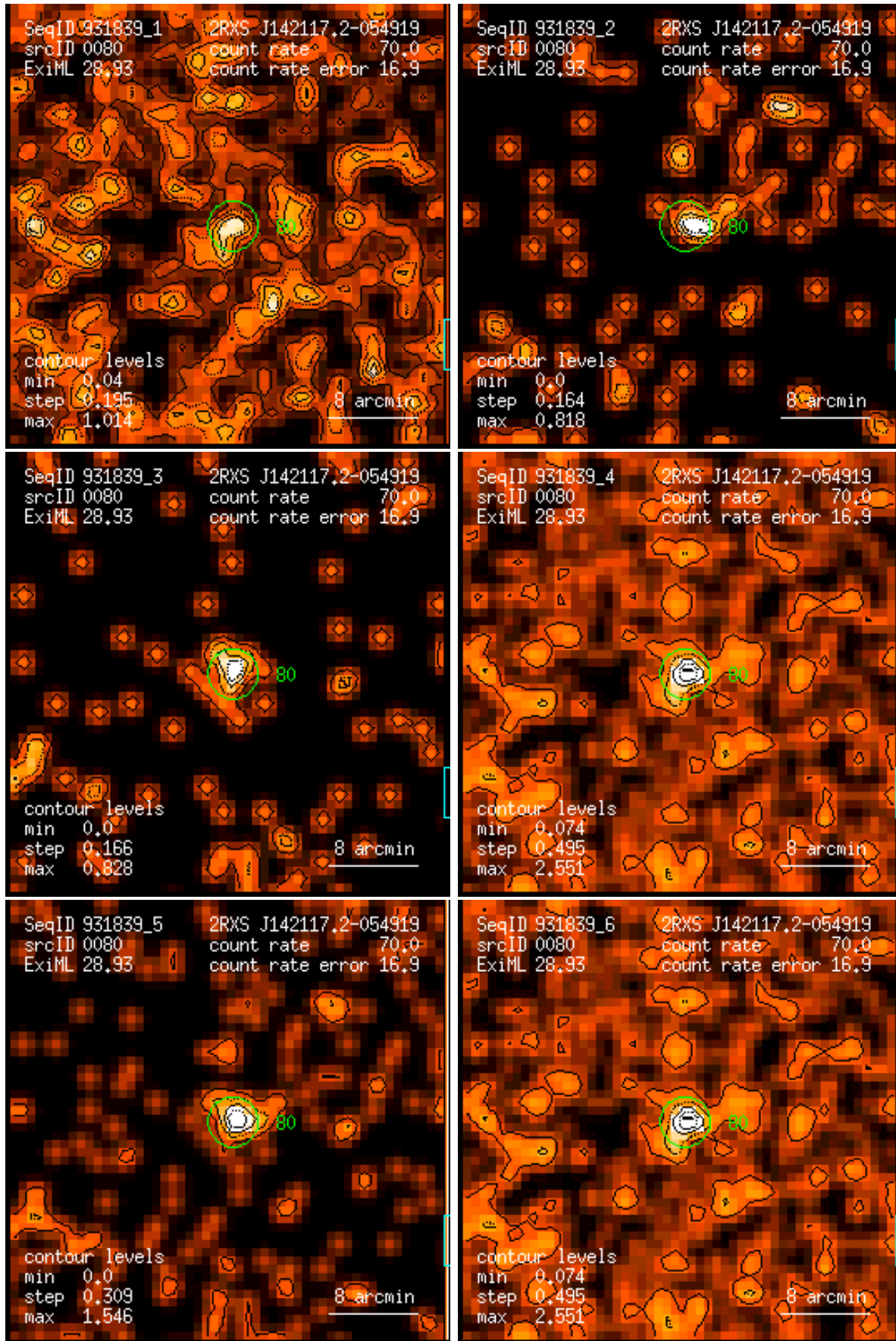
Figure 80: RASS 931839: detection 0080: band rate images, Gaussian filter: (1) PSPC channels 11 – 41, (2) 52 – 90, (3) 91 – 201, (4) 11 – 235, (5) 52 – 201, (6) 11 – 201. Broad band rates in counts/ks. Band rate contour levels in counts/ks/arcmin 2 .
