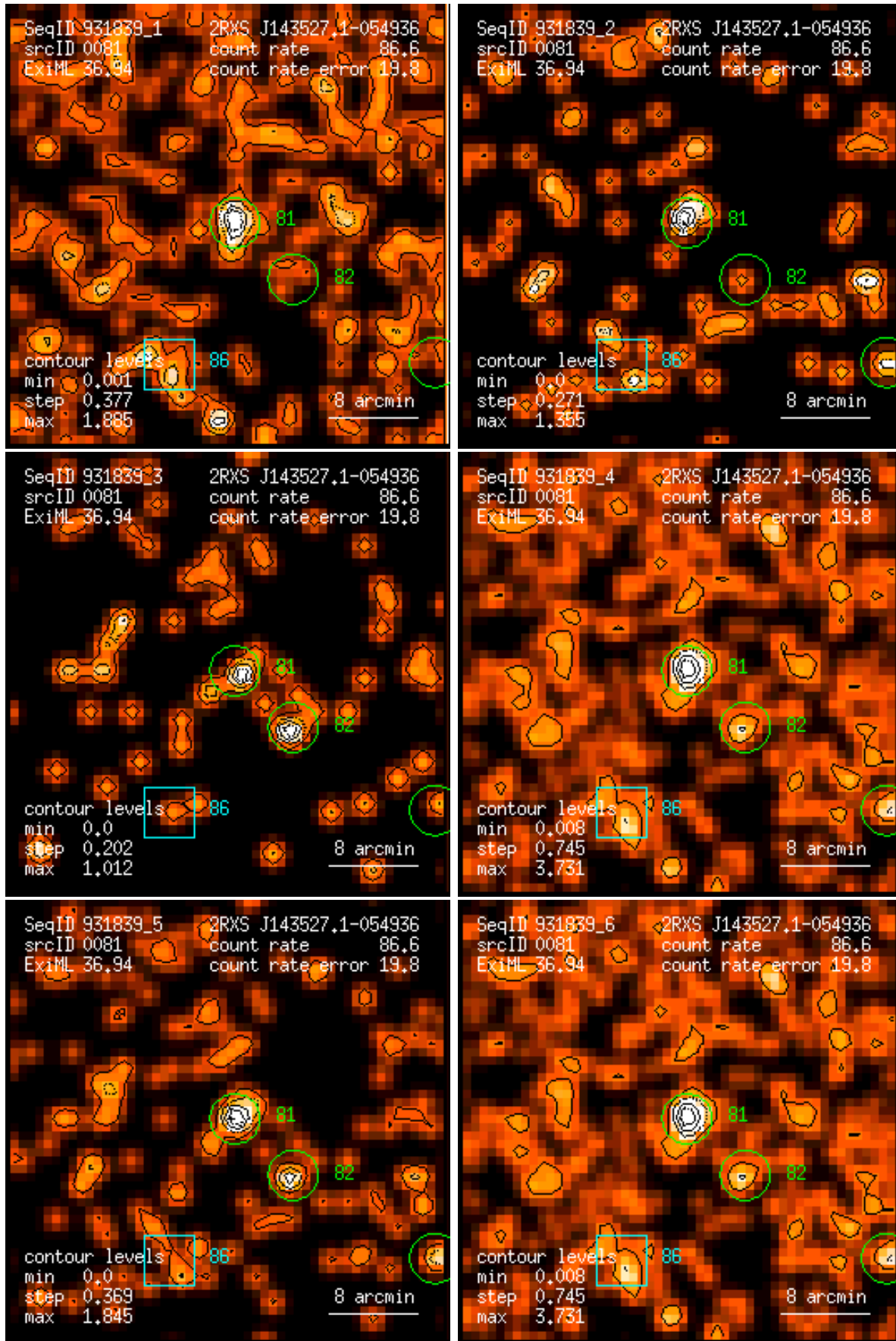
Figure 81: RASS 931839: detection 0081: band rate images, Gaussian filter: (1) PSPC channels 11 – 41, (2) 52 – 90, (3) 91 – 201, (4) 11 – 235, (5) 52 – 201, (6) 11 – 201. Broad band rates in counts/ks. Band rate contour levels in counts/ks/arcmin 2 .
