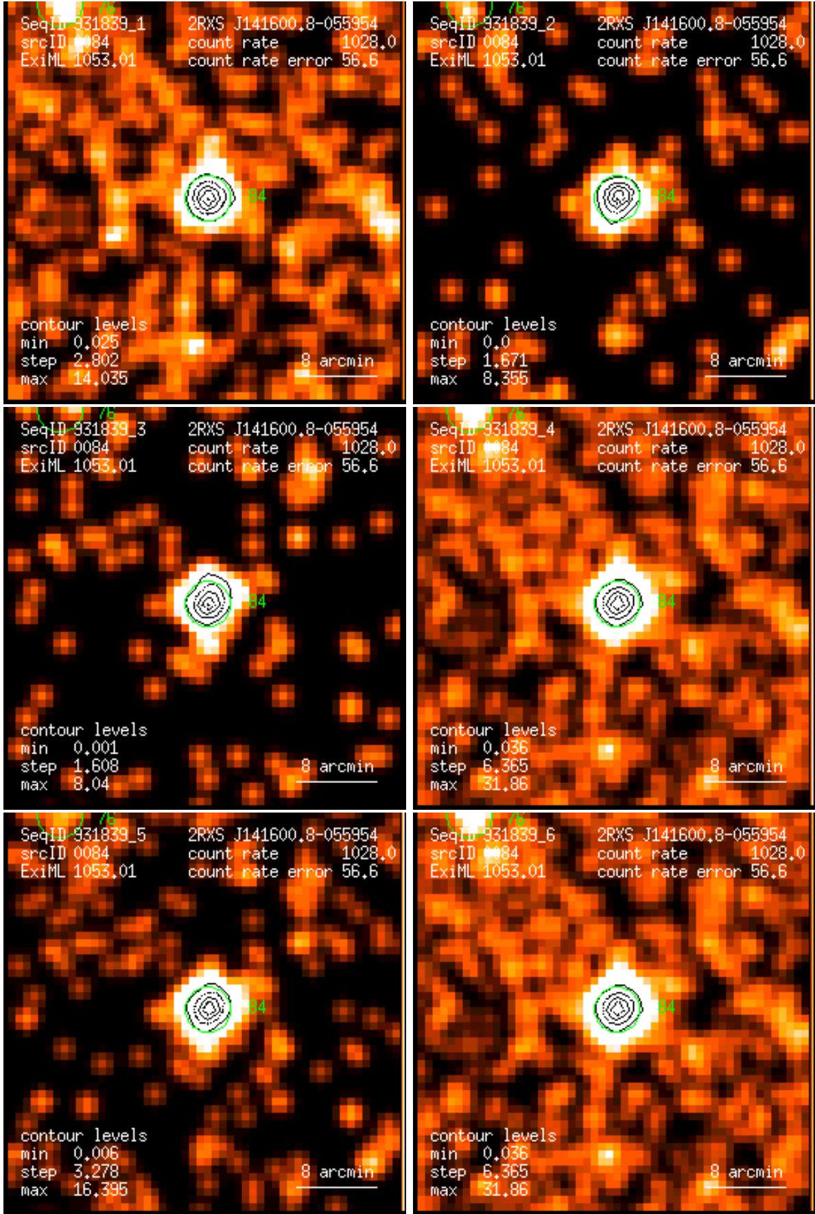
Figure 84: RASS 931839: detection 0084: band rate images, Gaussian filter: (1) PSPC channels 11 – 41, (2) 52 – 90, (3) 91 – 201, (4) 11 – 235, (5) 52 – 201, (6) 11 – 201. Broad band rates in counts/ks. Band rate contour levels in counts/ks/arcmin 2 .
