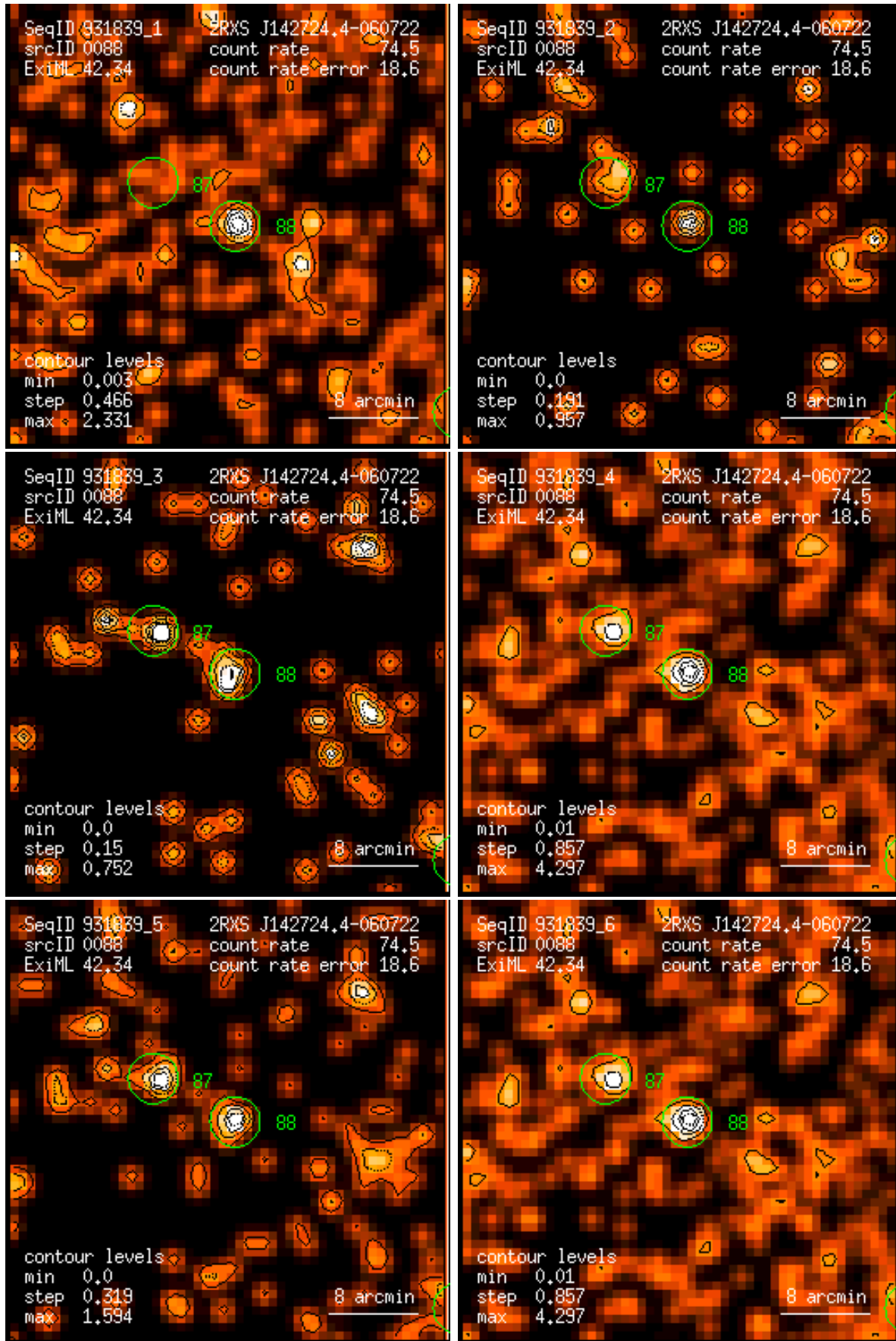
Figure 88: RASS 931839: detection 0088: band rate images, Gaussian filter: (1) PSPC channels 11 – 41, (2) 52 – 90, (3) 91 – 201, (4) 11 – 235, (5) 52 – 201, (6) 11 – 201. Broad band rates in counts/ks. Band rate contour levels in counts/ks/arcmin 2 .
