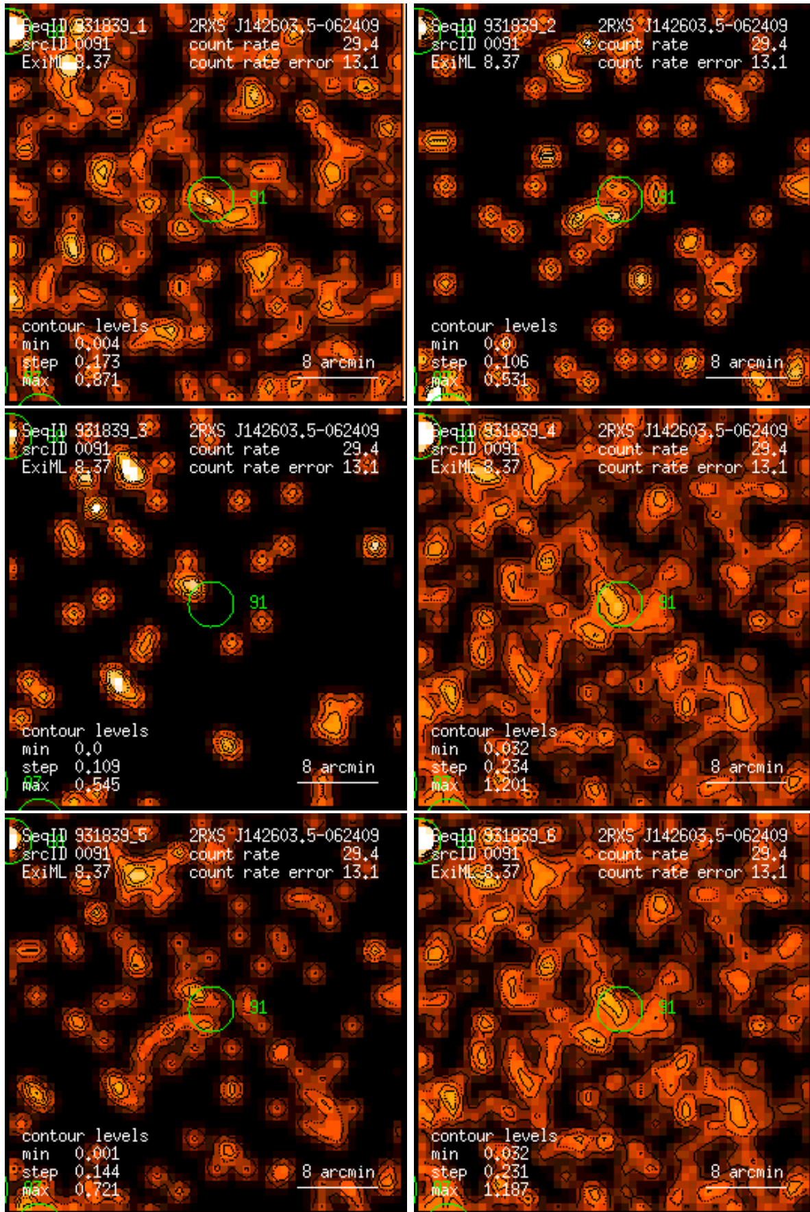
Figure 91: RASS 931839: detection 0091: band rate images, Gaussian filter: (1) PSPC channels 11 – 41, (2) 52 – 90, (3) 91 – 201, (4) 11 – 235, (5) 52 – 201, (6) 11 – 201. Broad band rates in counts/ks. Band rate contour levels in counts/ks/arcmin 2 .
