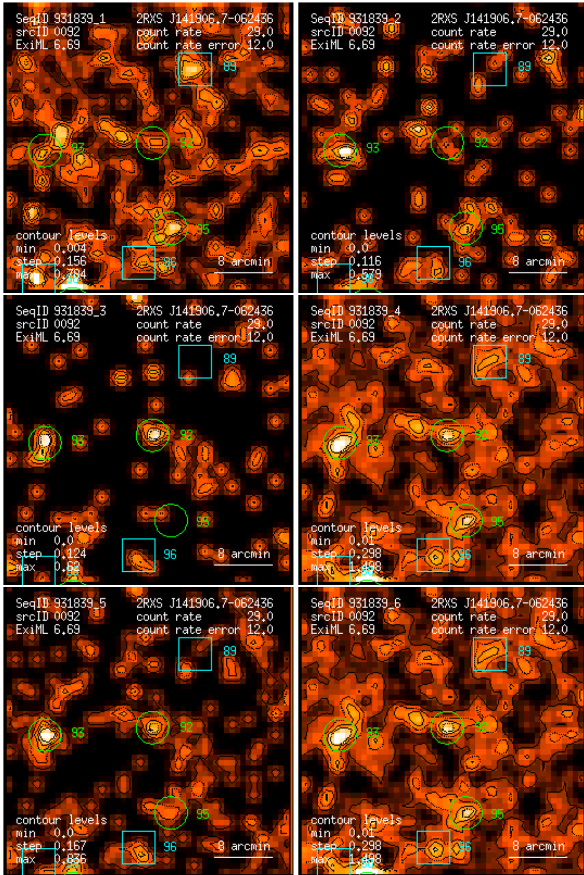
Figure 92: RASS 931839: detection 0092: band rate images, Gaussian filter: (1) PSPC channels 11 – 41, (2) 52 – 90, (3) 91 – 201, (4) 11 – 235, (5) 52 – 201, (6) 11 – 201. Broad band rates in counts/ks. Band rate contour levels in counts/ks/arcmin 2 .
