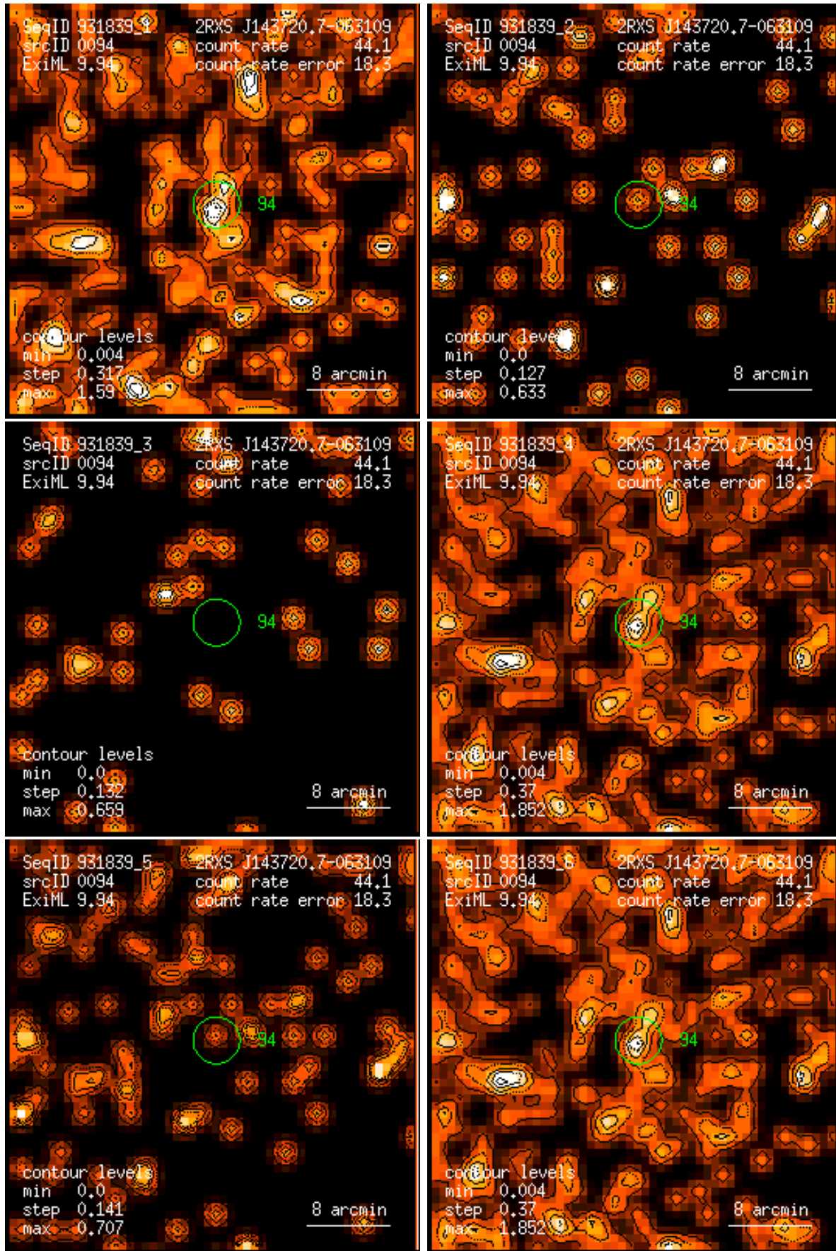
Figure 94: RASS 931839: detection 0094: band rate images, Gaussian filter: (1) PSPC channels 11 – 41, (2) 52 – 90, (3) 91 – 201, (4) 11 – 235, (5) 52 – 201, (6) 11 – 201. Broad band rates in counts/ks. Band rate contour levels in counts/ks/arcmin 2 .
