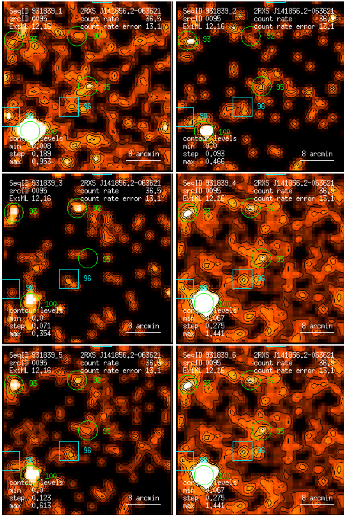
Figure 95: RASS 931839: detection 0095: band rate images, Gaussian filter: (1) PSPC channels 11 – 41, (2) 52 – 90, (3) 91 – 201, (4) 11 – 235, (5) 52 – 201, (6) 11 – 201. Broad band rates in counts/ks. Band rate contour levels in counts/ks/arcmin 2 .
