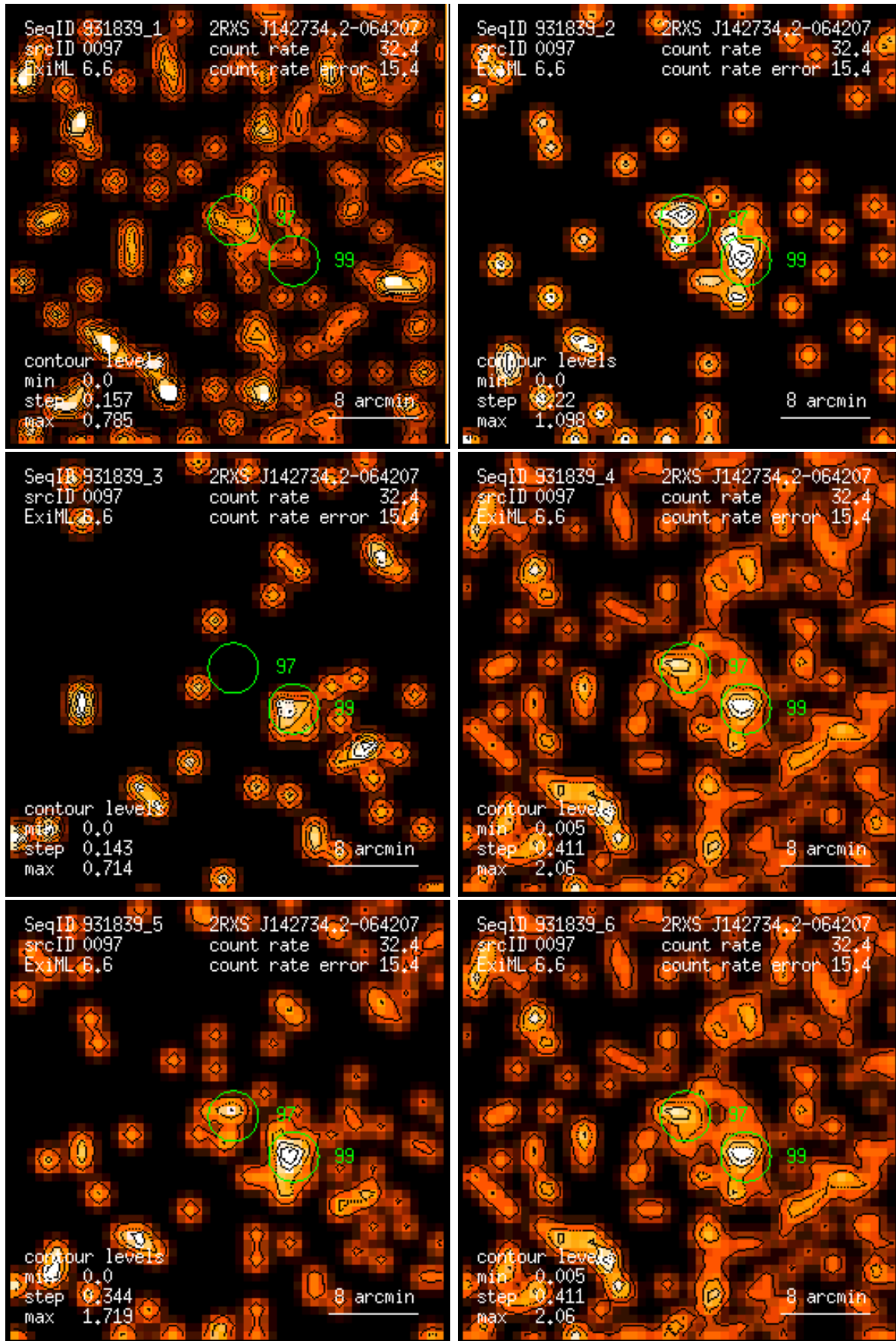
Figure 97: RASS 931839: detection 0097: band rate images, Gaussian filter: (1) PSPC channels 11 – 41, (2) 52 – 90, (3) 91 – 201, (4) 11 – 235, (5) 52 – 201, (6) 11 – 201. Broad band rates in counts/ks. Band rate contour levels in counts/ks/arcmin 2 .
