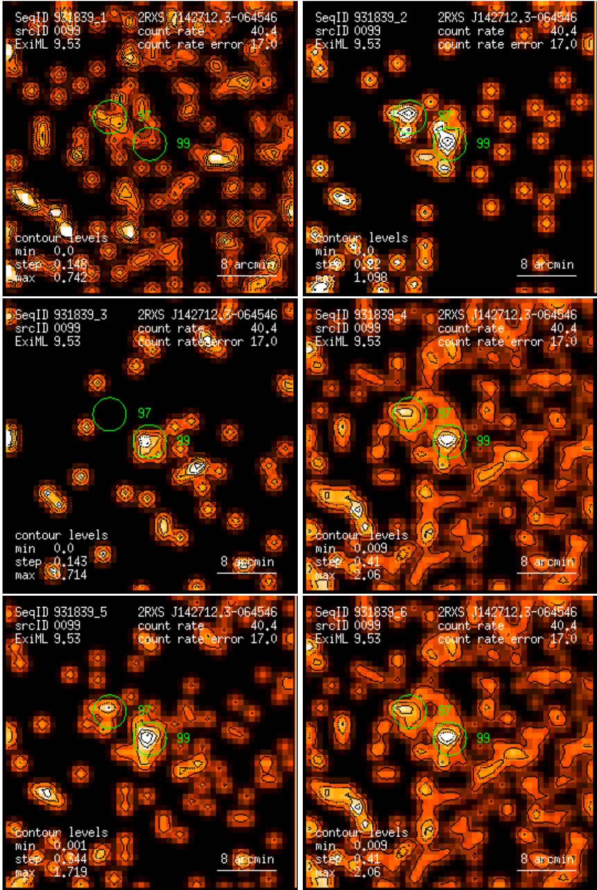
Figure 99: RASS 931839: detection 0099: band rate images, Gaussian filter: (1) PSPC channels 11 – 41, (2) 52 – 90, (3) 91 – 201, (4) 11 – 235, (5) 52 – 201, (6) 11 – 201. Broad band rates in counts/ks. Band rate contour levels in counts/ks/arcmin 2 .
