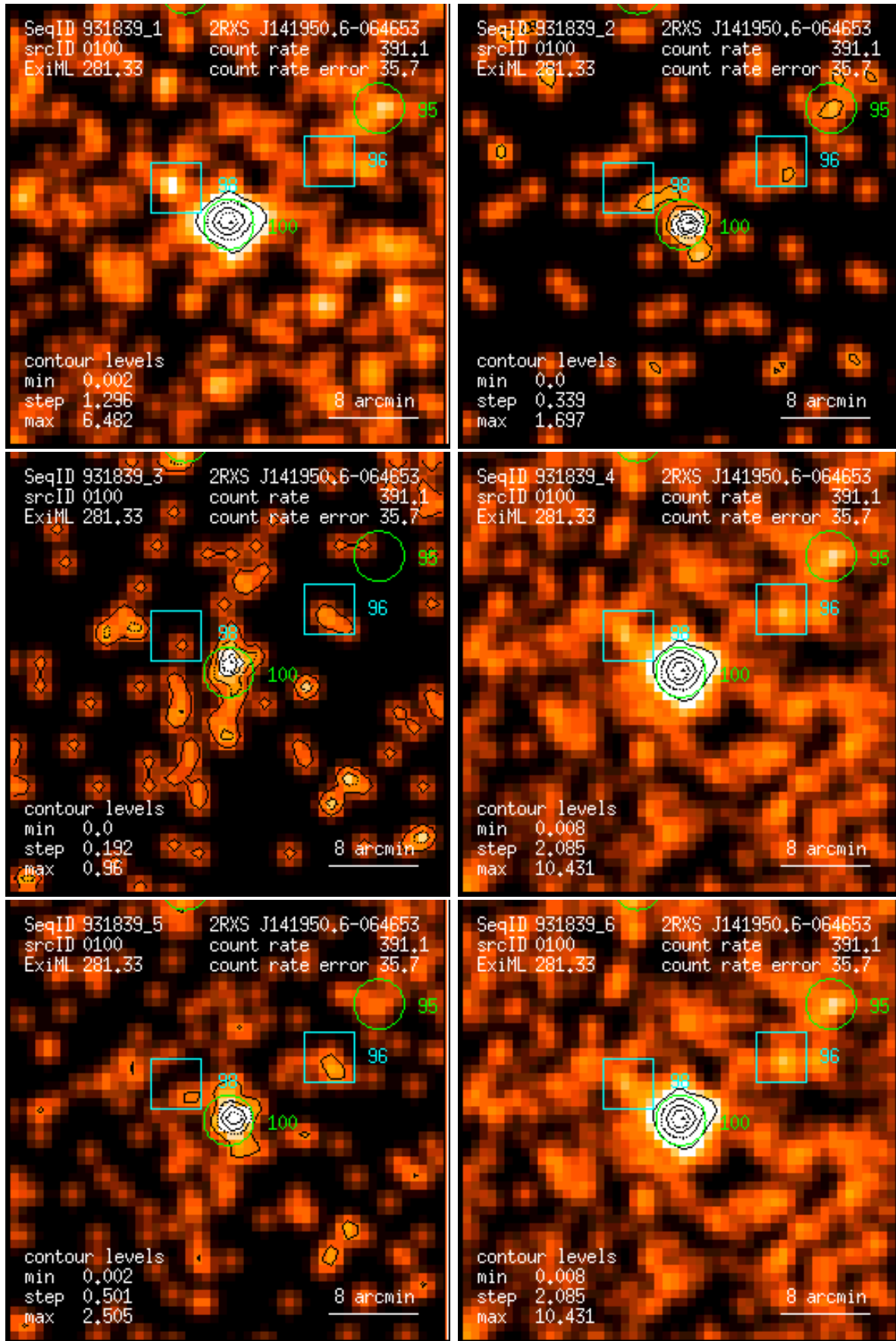
Figure 100: RASS 931839: detection 0100: band rate images, Gaussian filter: (1) PSPC channels 11 – 41, (2) 52 – 90, (3) 91 – 201, (4) 11 – 235, (5) 52 – 201, (6) 11 – 201. Broad band rates in counts/ks. Band rate contour levels in counts/ks/arcmin 2 .
