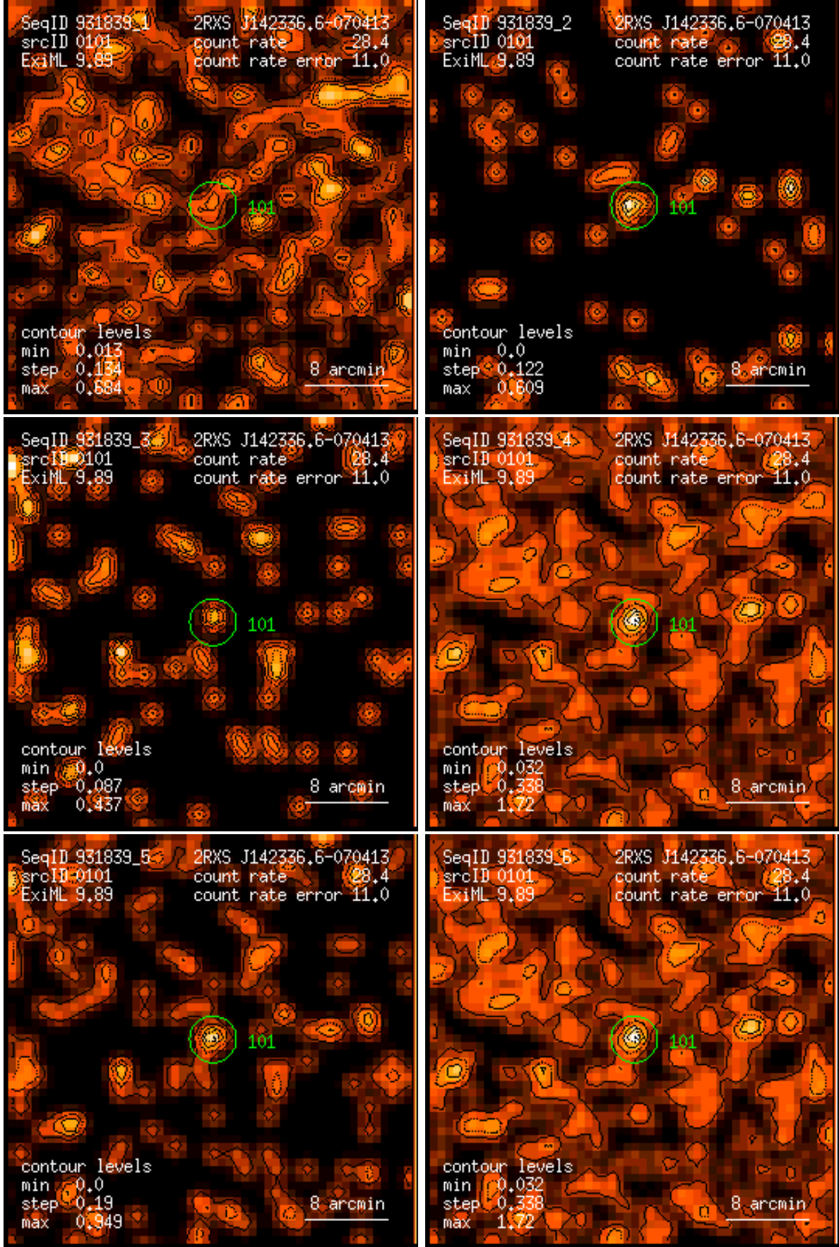
Figure 101: RASS 931839: detection 0101: band rate images, Gaussian filter: (1) PSPC channels 11 – 41, (2) 52 – 90, (3) 91 – 201, (4) 11 – 235, (5) 52 – 201, (6) 11 – 201. Broad band rates in counts/ks. Band rate contour levels in counts/ks/arcmin 2 .
