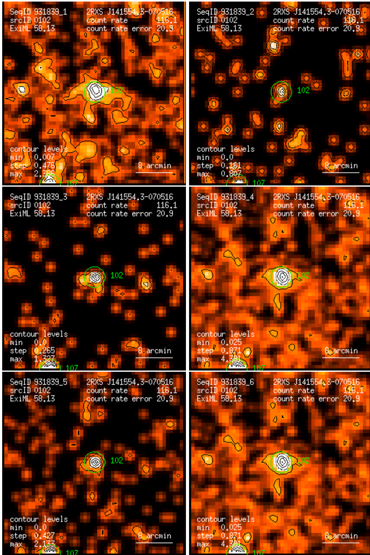
Figure 102: RASS 931839: detection 0102: band rate images, Gaussian filter: (1) PSPC channels 11 – 41, (2) 52 – 90, (3) 91 – 201, (4) 11 – 235, (5) 52 – 201, (6) 11 – 201. Broad band rates in counts/ks. Band rate contour levels in counts/ks/arcmin 2 .
