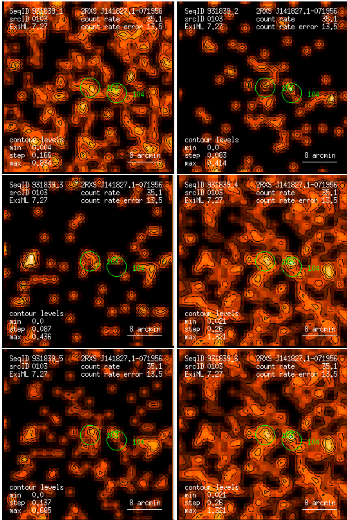
Figure 103: RASS 931839: detection 0103: band rate images, Gaussian filter: (1) PSPC channels 11 – 41, (2) 52 – 90, (3) 91 – 201, (4) 11 – 235, (5) 52 – 201, (6) 11 – 201. Broad band rates in counts/ks. Band rate contour levels in counts/ks/arcmin 2 .
