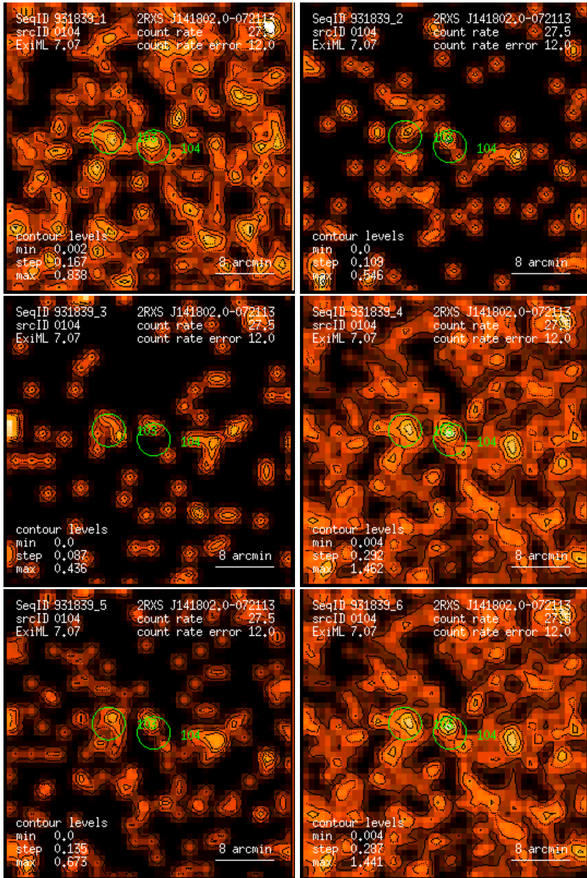
Figure 104: RASS 931839: detection 0104: band rate images, Gaussian filter: (1) PSPC channels 11 – 41, (2) 52 – 90, (3) 91 – 201, (4) 11 – 235, (5) 52 – 201, (6) 11 – 201. Broad band rates in counts/ks. Band rate contour levels in counts/ks/arcmin 2 .
