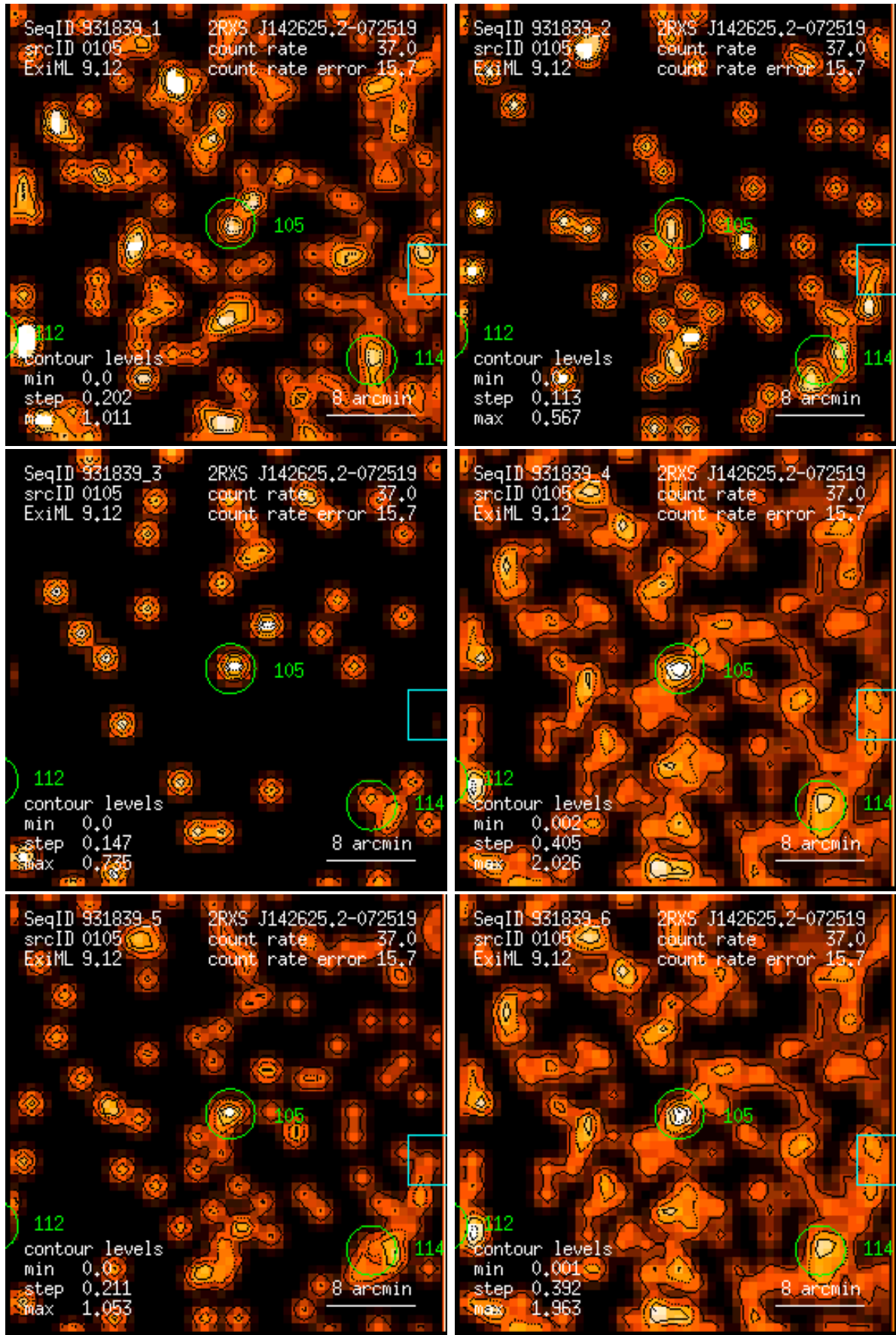
Figure 105: RASS 931839: detection 0105: band rate images, Gaussian filter: (1) PSPC channels 11 – 41, (2) 52 – 90, (3) 91 – 201, (4) 11 – 235, (5) 52 – 201, (6) 11 – 201. Broad band rates in counts/ks. Band rate contour levels in counts/ks/arcmin 2 .
