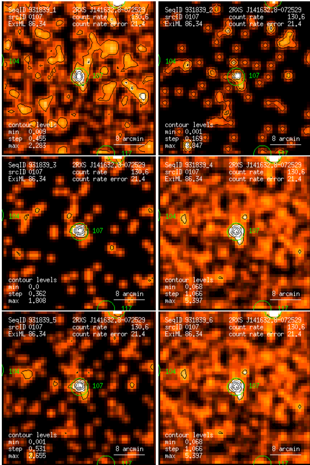
Figure 107: RASS 931839: detection 0107: band rate images, Gaussian filter: (1) PSPC channels 11 – 41, (2) 52 – 90, (3) 91 – 201, (4) 11 – 235, (5) 52 – 201, (6) 11 – 201. Broad band rates in counts/ks. Band rate contour levels in counts/ks/arcmin 2 .
