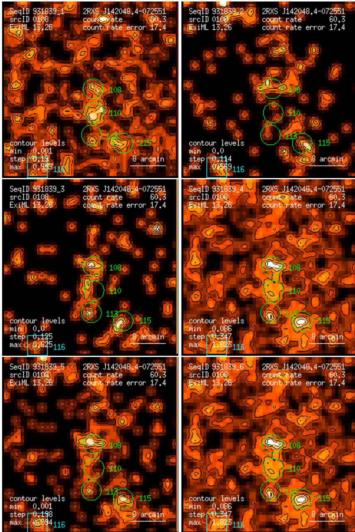
Figure 108: RASS 931839: detection 0108: band rate images, Gaussian filter: (1) PSPC channels 11 – 41, (2) 52 – 90, (3) 91 – 201, (4) 11 – 235, (5) 52 – 201, (6) 11 – 201. Broad band rates in counts/ks. Band rate contour levels in counts/ks/arcmin 2 .
