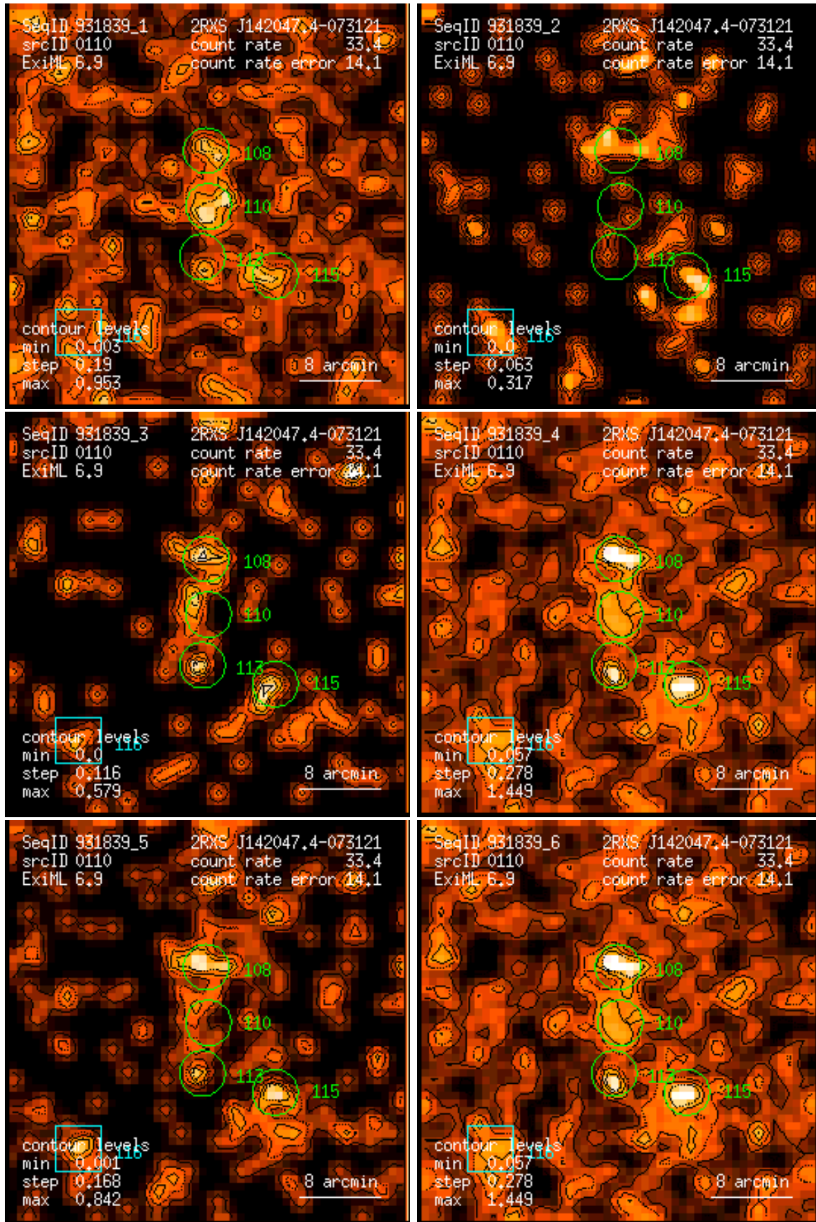
Figure 110: RASS 931839: detection 0110: band rate images, Gaussian filter: (1) PSPC channels 11 – 41, (2) 52 – 90, (3) 91 – 201, (4) 11 – 235, (5) 52 – 201, (6) 11 – 201. Broad band rates in counts/ks. Band rate contour levels in counts/ks/arcmin 2 .
