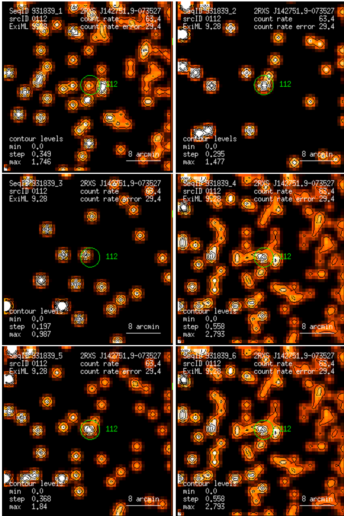
Figure 112: RASS 931839: detection 0112: band rate images, Gaussian filter: (1) PSPC channels 11 – 41, (2) 52 – 90, (3) 91 – 201, (4) 11 – 235, (5) 52 – 201, (6) 11 – 201. Broad band rates in counts/ks. Band rate contour levels in counts/ks/arcmin 2 .
