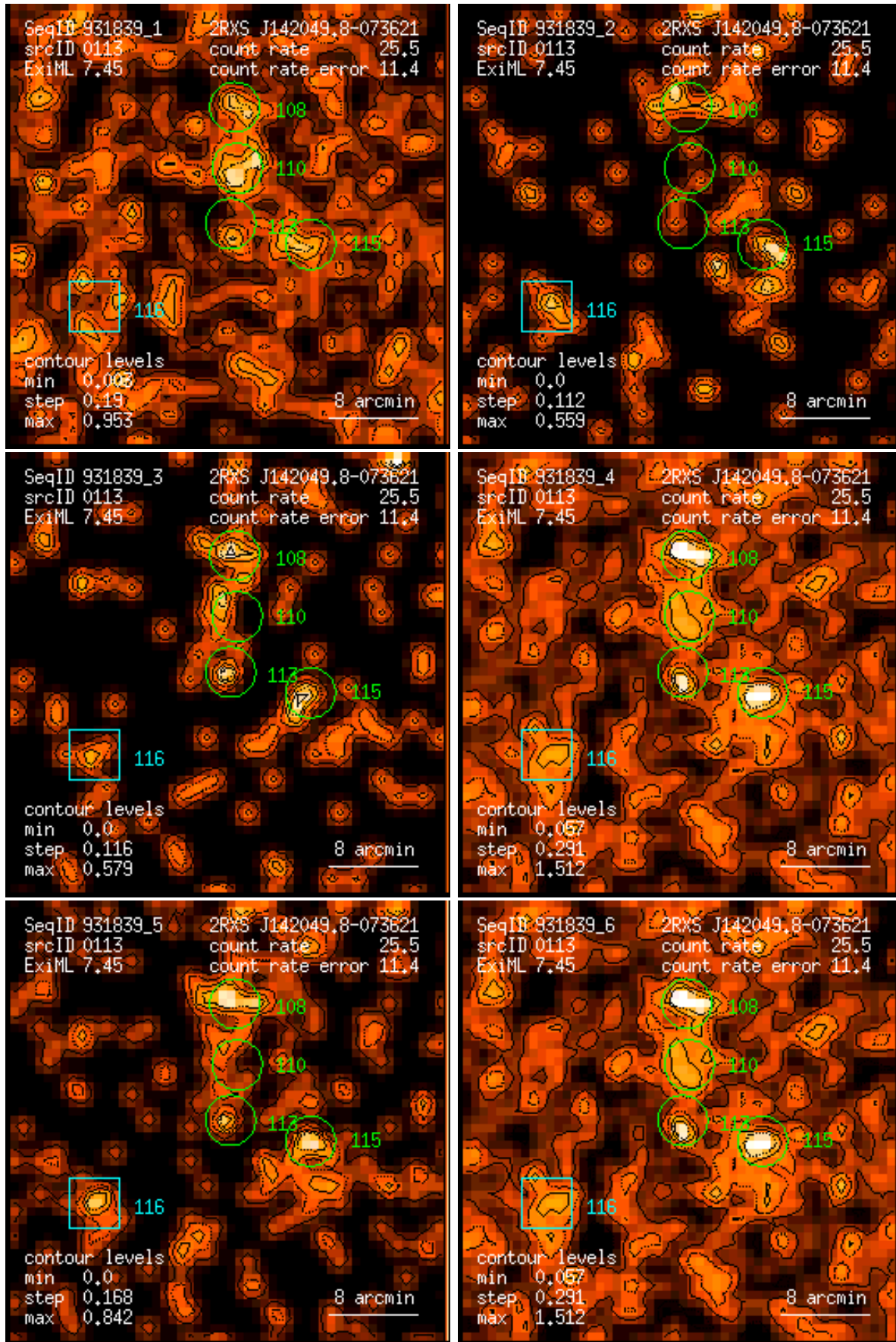
Figure 113: RASS 931839: detection 0113: band rate images, Gaussian filter: (1) PSPC channels 11 – 41, (2) 52 – 90, (3) 91 – 201, (4) 11 – 235, (5) 52 – 201, (6) 11 – 201. Broad band rates in counts/ks. Band rate contour levels in counts/ks/arcmin 2 .
