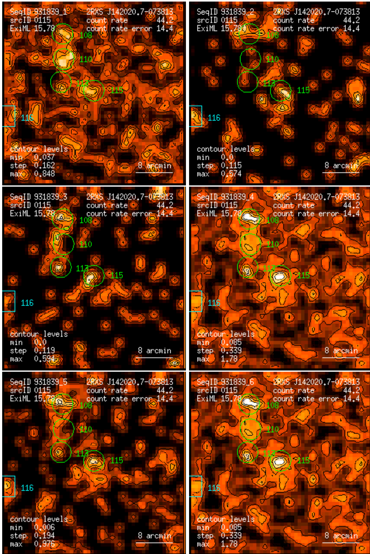
Figure 115: RASS 931839: detection 0115: band rate images, Gaussian filter: (1) PSPC channels 11 – 41, (2) 52 – 90, (3) 91 – 201, (4) 11 – 235, (5) 52 – 201, (6) 11 – 201. Broad band rates in counts/ks. Band rate contour levels in counts/ks/arcmin 2 .
