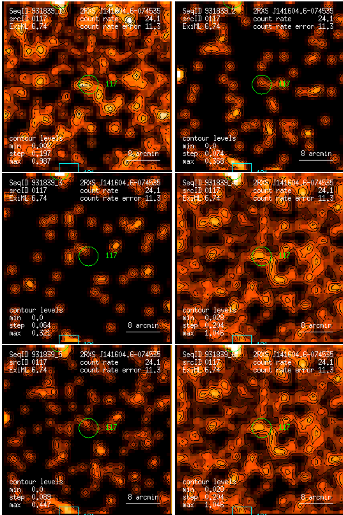
Figure 117: RASS 931839: detection 0117: band rate images, Gaussian filter: (1) PSPC channels 11 – 41, (2) 52 – 90, (3) 91 – 201, (4) 11 – 235, (5) 52 – 201, (6) 11 – 201. Broad band rates in counts/ks. Band rate contour levels in counts/ks/arcmin 2 .
