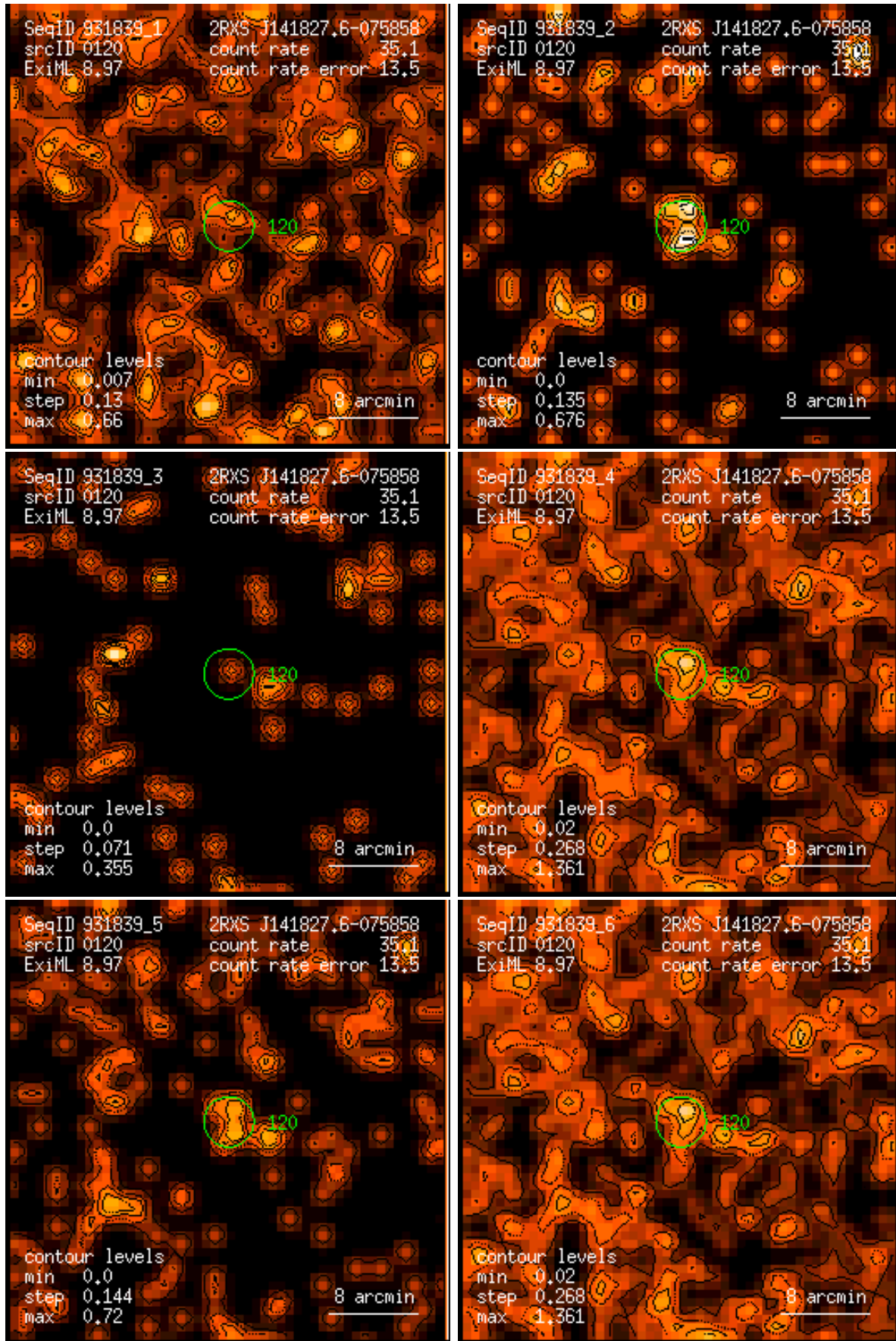
Figure 120: RASS 931839: detection 0120: band rate images, Gaussian filter: (1) PSPC channels 11 – 41, (2) 52 – 90, (3) 91 – 201, (4) 11 – 235, (5) 52 – 201, (6) 11 – 201. Broad band rates in counts/ks. Band rate contour levels in counts/ks/arcmin 2 .
