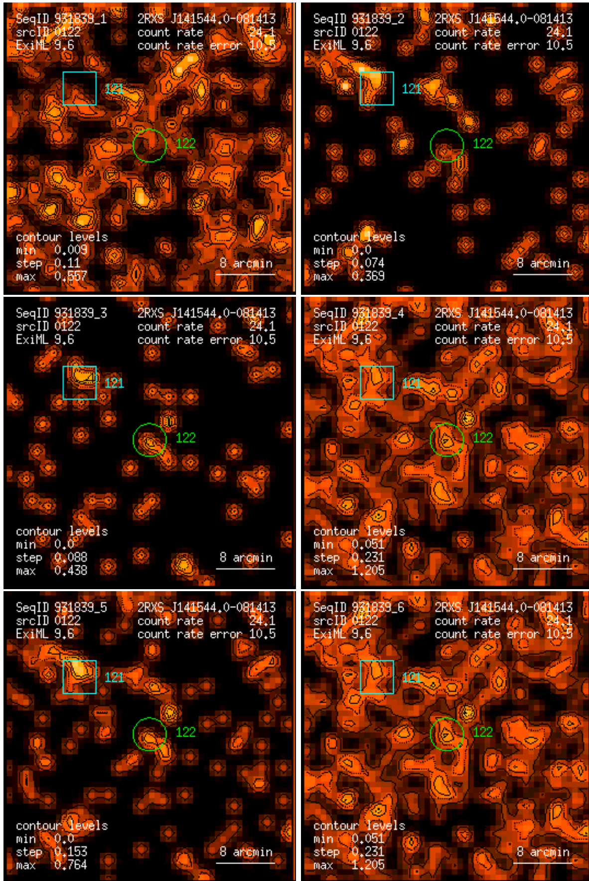
Figure 122: RASS 931839: detection 0122: band rate images, Gaussian filter: (1) PSPC channels 11 – 41, (2) 52 – 90, (3) 91 – 201, (4) 11 – 235, (5) 52 – 201, (6) 11 – 201. Broad band rates in counts/ks. Band rate contour levels in counts/ks/arcmin 2 .
