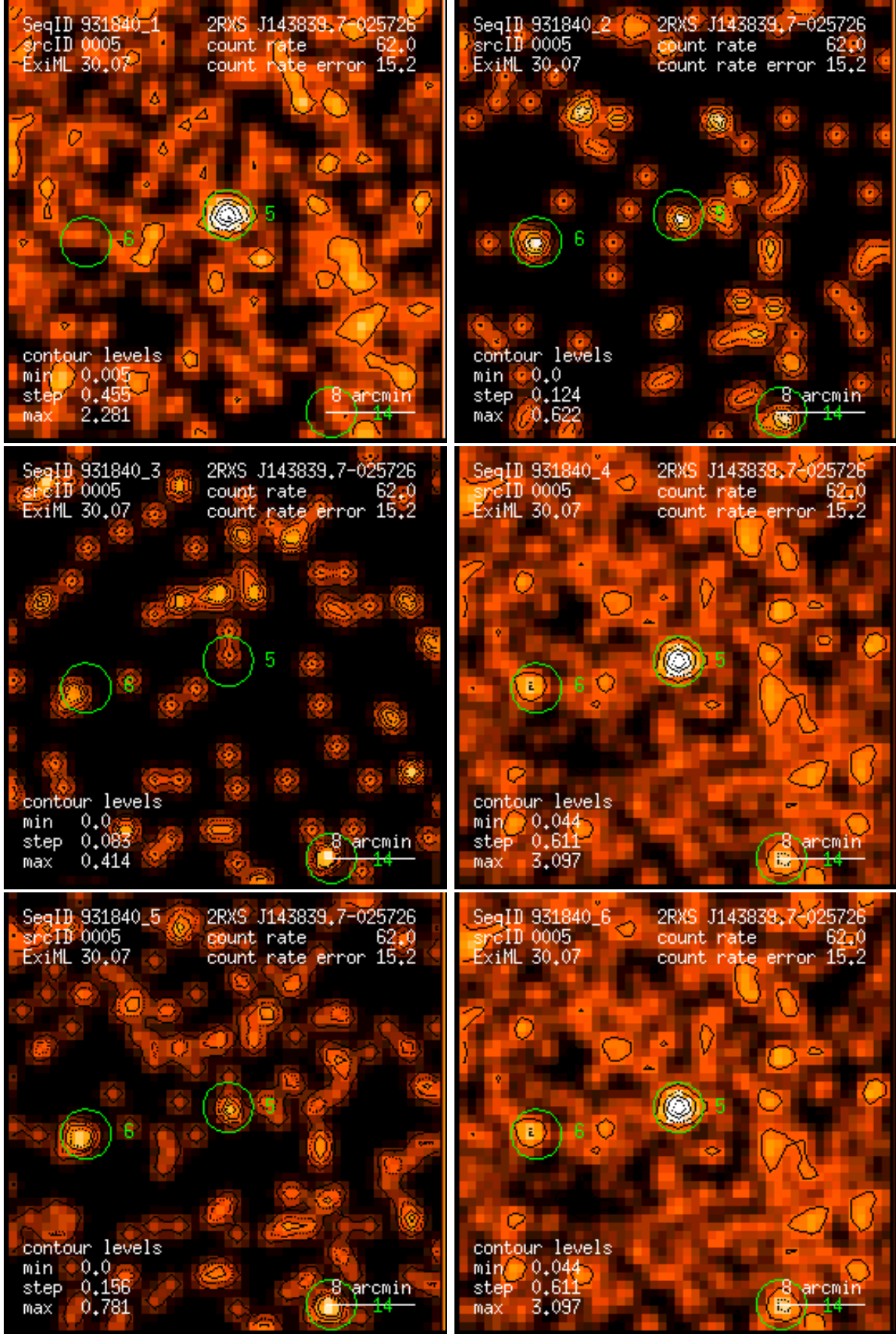
Figure 5: RASS 931840: detection 0005: band rate images, Gaussian filter: (1) PSPC channels 11 – 41, (2) 52 – 90, (3) 91 – 201, (4) 11 – 235, (5) 52 – 201, (6) 11 – 201. Broad band rates in counts/ks. Band rate contour levels in counts/ks/arcmin 2 .
