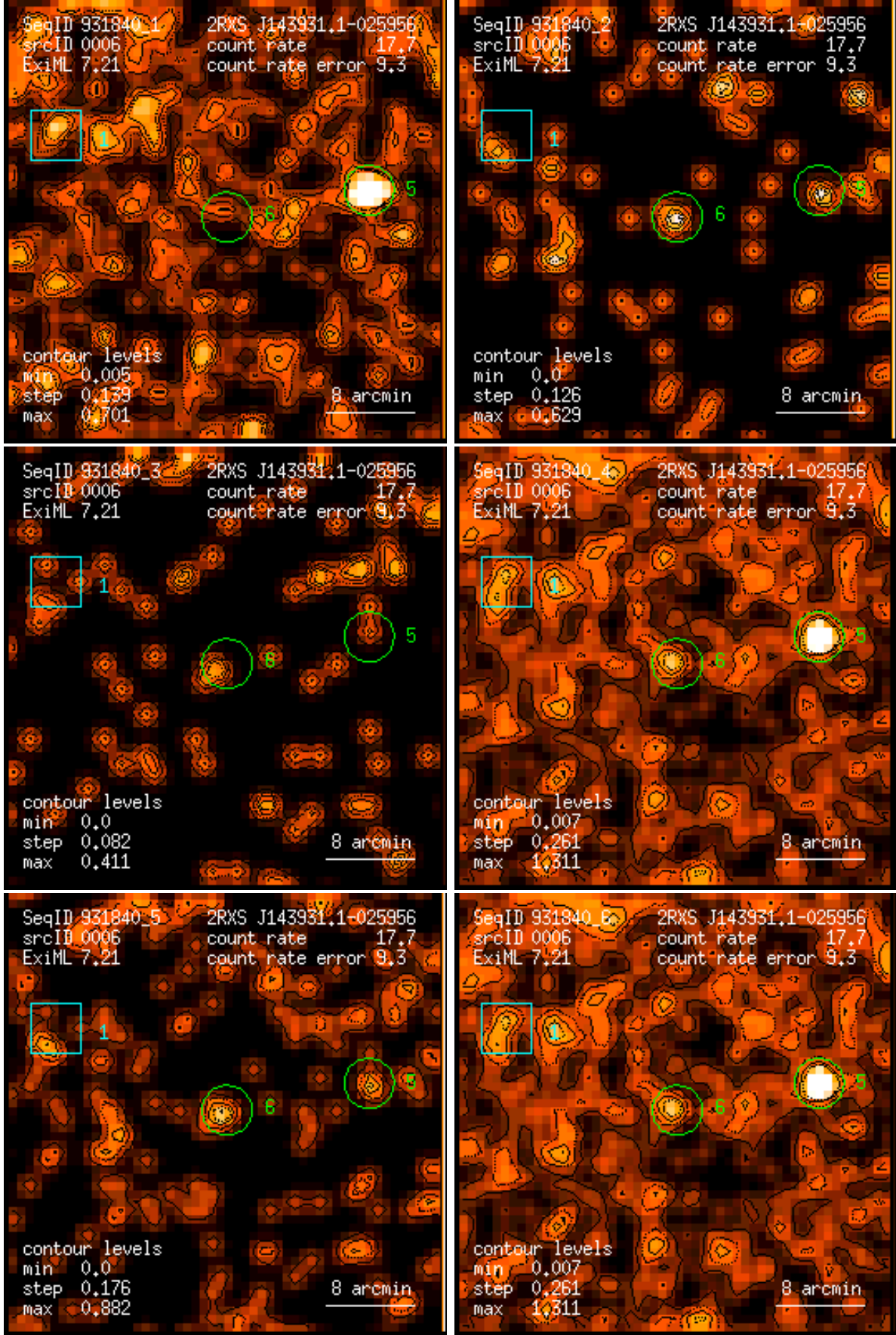
Figure 6: RASS 931840: detection 0006: band rate images, Gaussian filter: (1) PSPC channels 11 – 41, (2) 52 – 90, (3) 91 – 201, (4) 11 – 235, (5) 52 – 201, (6) 11 – 201. Broad band rates in counts/ks. Band rate contour levels in counts/ks/arcmin 2 .
