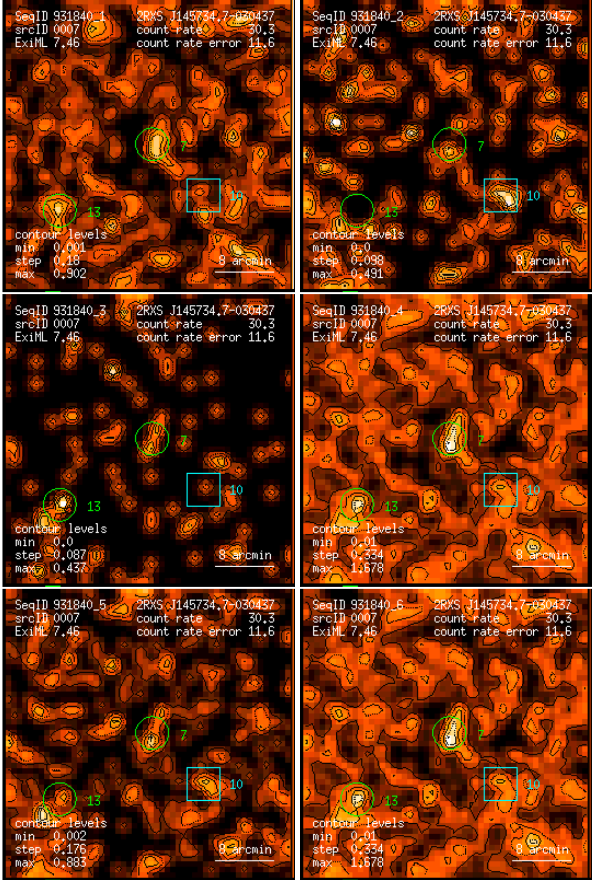
Figure 7: RASS 931840: detection 0007: band rate images, Gaussian filter: (1) PSPC channels 11 – 41, (2) 52 – 90, (3) 91 – 201, (4) 11 – 235, (5) 52 – 201, (6) 11 – 201. Broad band rates in counts/ks. Band rate contour levels in counts/ks/arcmin 2 .
