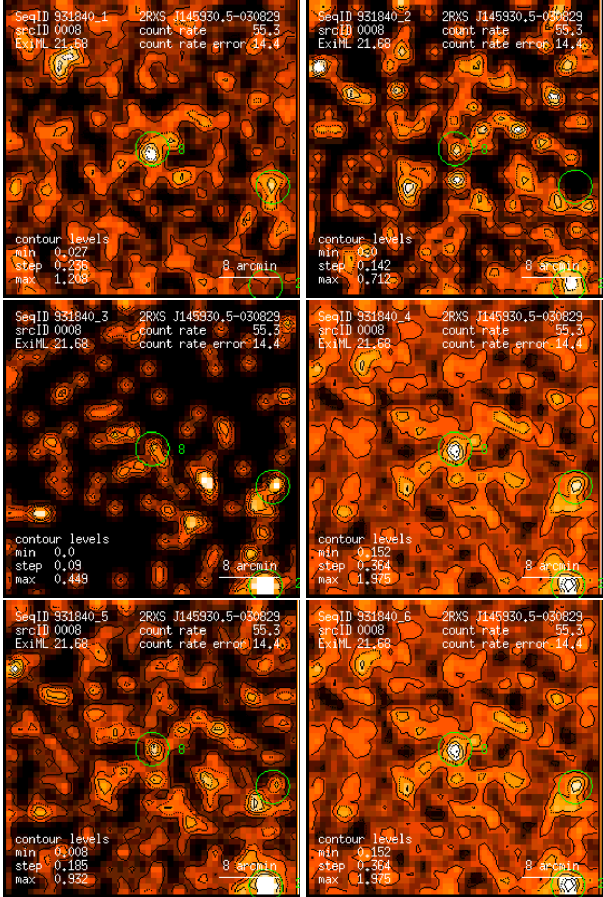
Figure 8: RASS 931840: detection 0008: band rate images, Gaussian filter: (1) PSPC channels 11 – 41, (2) 52 – 90, (3) 91 – 201, (4) 11 – 235, (5) 52 – 201, (6) 11 – 201. Broad band rates in counts/ks. Band rate contour levels in counts/ks/arcmin 2 .
