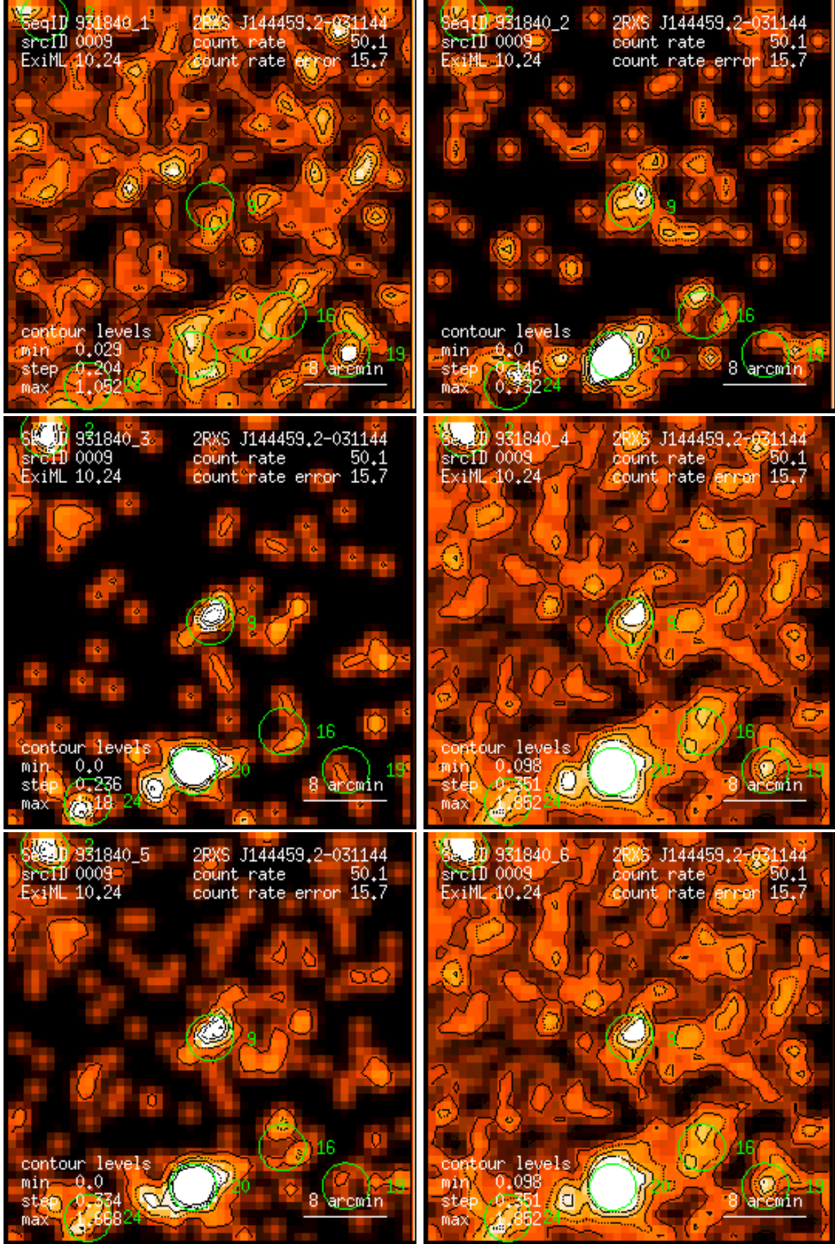
Figure 9: RASS 931840: detection 0009: band rate images, Gaussian filter: (1) PSPC channels 11 – 41, (2) 52 – 90, (3) 91 – 201, (4) 11 – 235, (5) 52 – 201, (6) 11 – 201. Broad band rates in counts/ks. Band rate contour levels in counts/ks/arcmin 2 .
