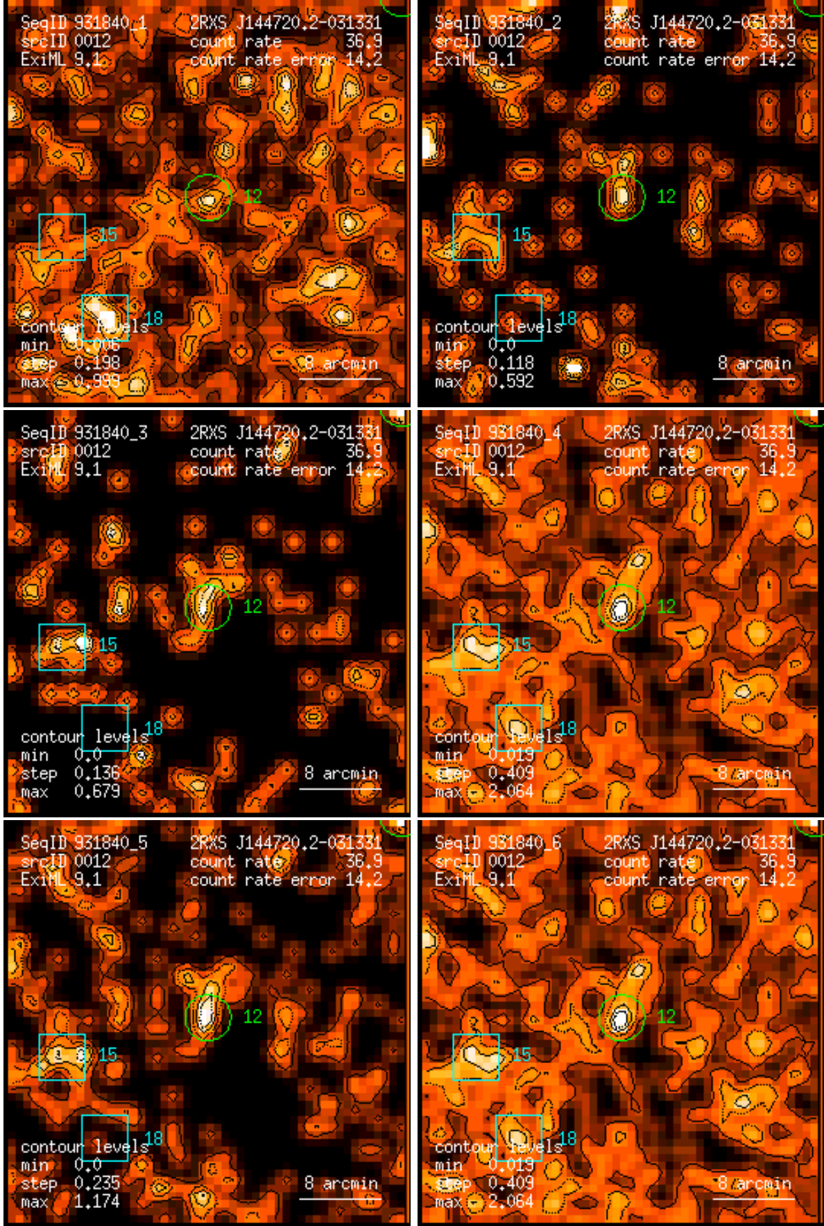
Figure 12: RASS 931840: detection 0012: band rate images, Gaussian filter: (1) PSPC channels 11 – 41, (2) 52 – 90, (3) 91 – 201, (4) 11 – 235, (5) 52 – 201, (6) 11 – 201. Broad band rates in counts/ks. Band rate contour levels in counts/ks/arcmin 2 .
