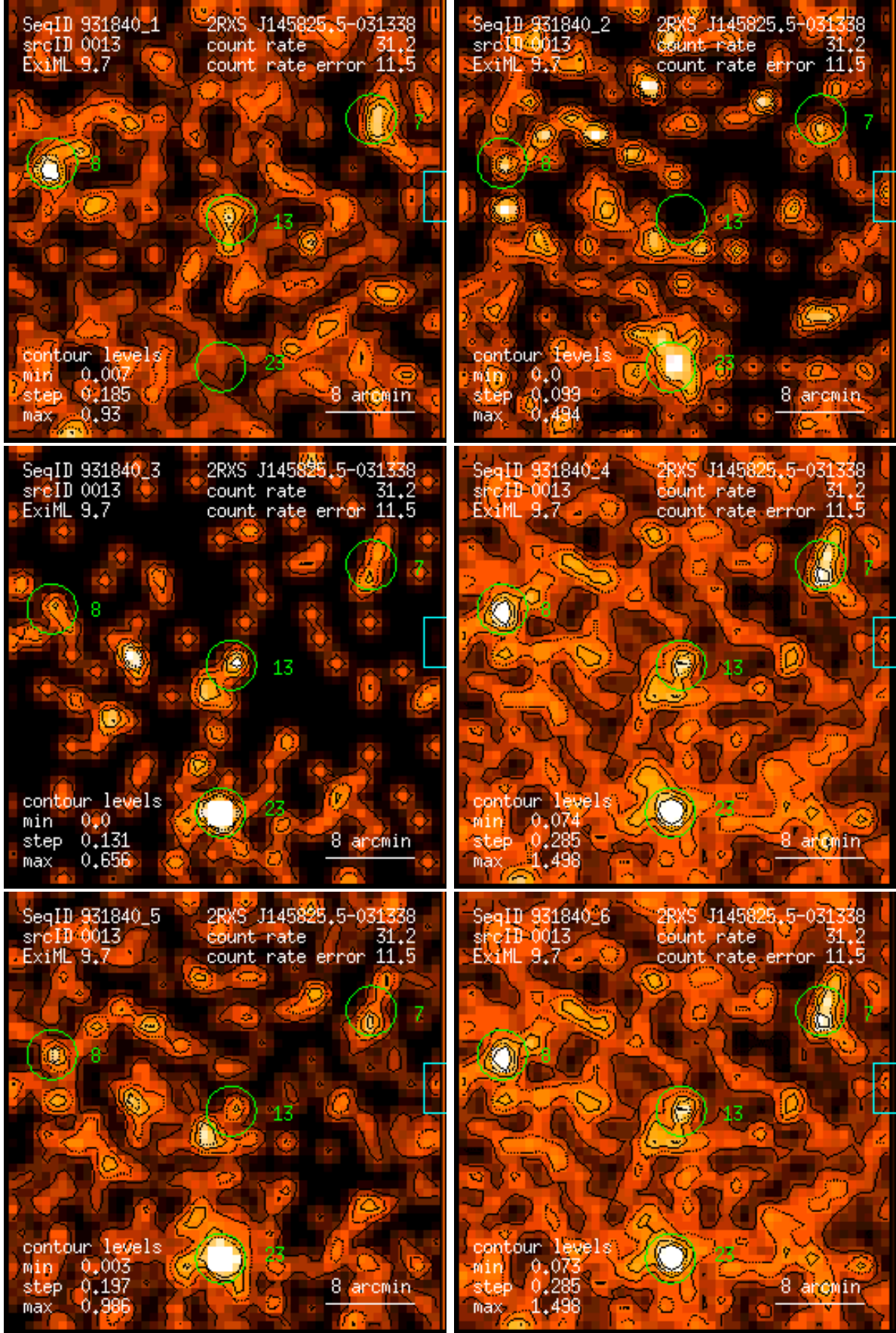
Figure 13: RASS 931840: detection 0013: band rate images, Gaussian filter: (1) PSPC channels 11 – 41, (2) 52 – 90, (3) 91 – 201, (4) 11 – 235, (5) 52 – 201, (6) 11 – 201. Broad band rates in counts/ks. Band rate contour levels in counts/ks/arcmin 2 .
