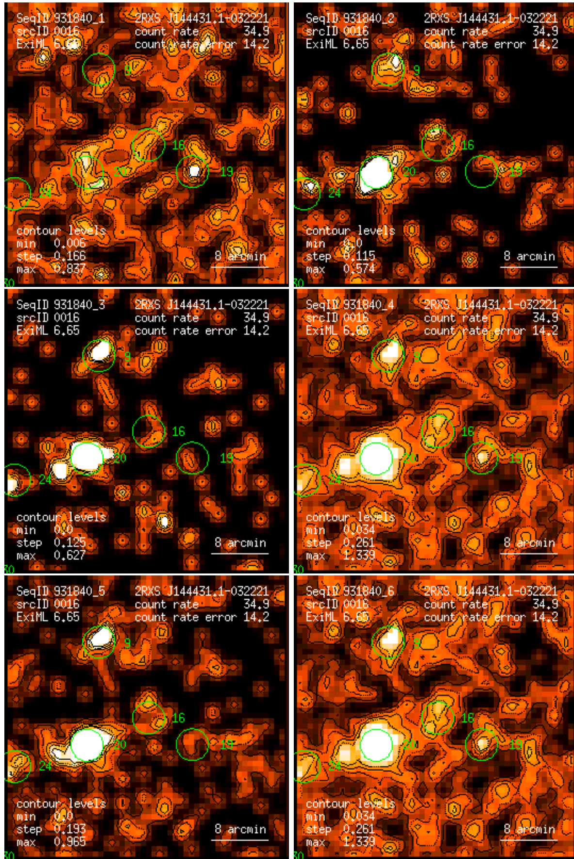
Figure 16: RASS 931840: detection 0016: band rate images, Gaussian filter: (1) PSPC channels 11 – 41, (2) 52 – 90, (3) 91 – 201, (4) 11 – 235, (5) 52 – 201, (6) 11 – 201. Broad band rates in counts/ks. Band rate contour levels in counts/ks/arcmin 2 .
