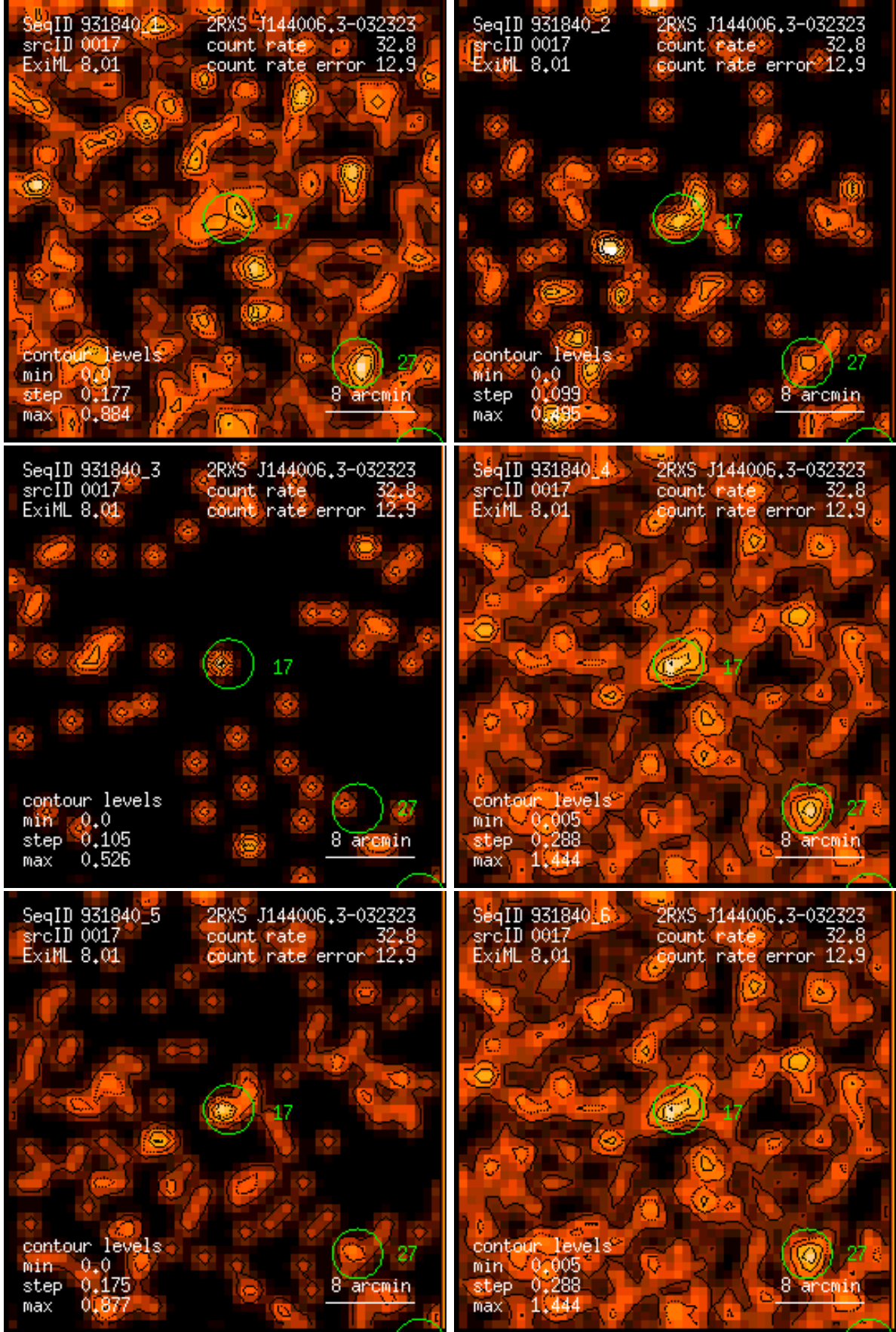
Figure 17: RASS 931840: detection 0017: band rate images, Gaussian filter: (1) PSPC channels 11 – 41, (2) 52 – 90, (3) 91 – 201, (4) 11 – 235, (5) 52 – 201, (6) 11 – 201. Broad band rates in counts/ks. Band rate contour levels in counts/ks/arcmin 2 .
