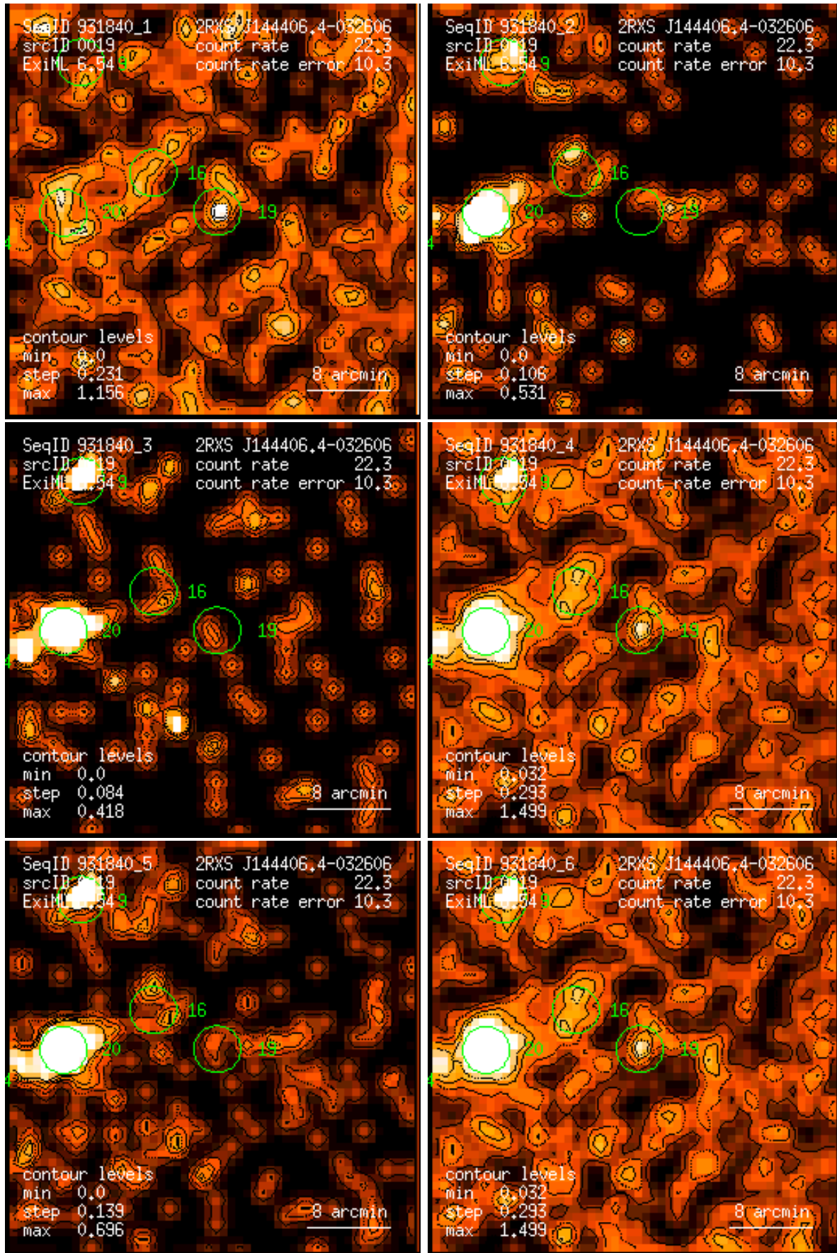
Figure 19: RASS 931840: detection 0019: band rate images, Gaussian filter: (1) PSPC channels 11 – 41, (2) 52 – 90, (3) 91 – 201, (4) 11 – 235, (5) 52 – 201, (6) 11 – 201. Broad band rates in counts/ks. Band rate contour levels in counts/ks/arcmin 2 .
