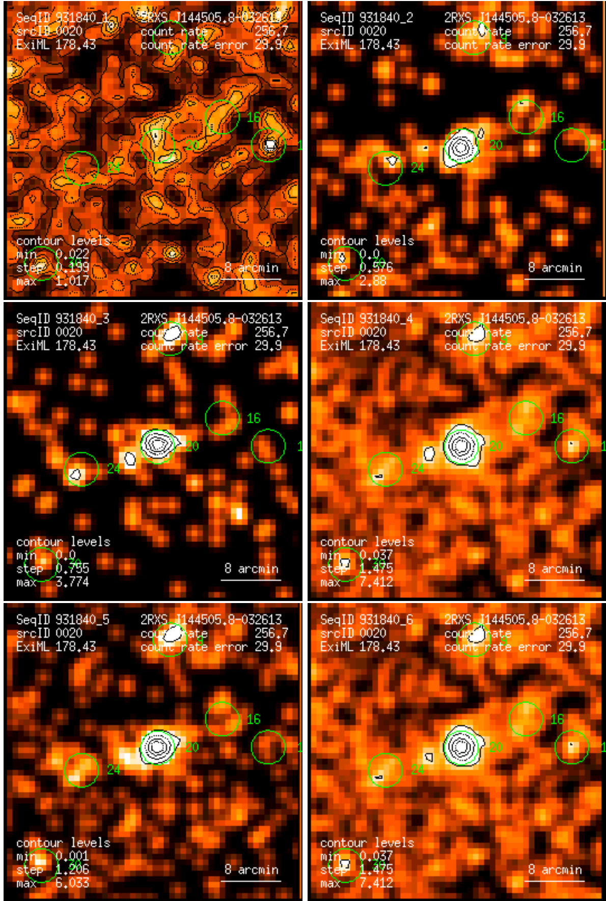
Figure 20: RASS 931840: detection 0020: band rate images, Gaussian filter: (1) PSPC channels 11 – 41, (2) 52 – 90, (3) 91 – 201, (4) 11 – 235, (5) 52 – 201, (6) 11 – 201. Broad band rates in counts/ks. Band rate contour levels in counts/ks/arcmin 2 .
