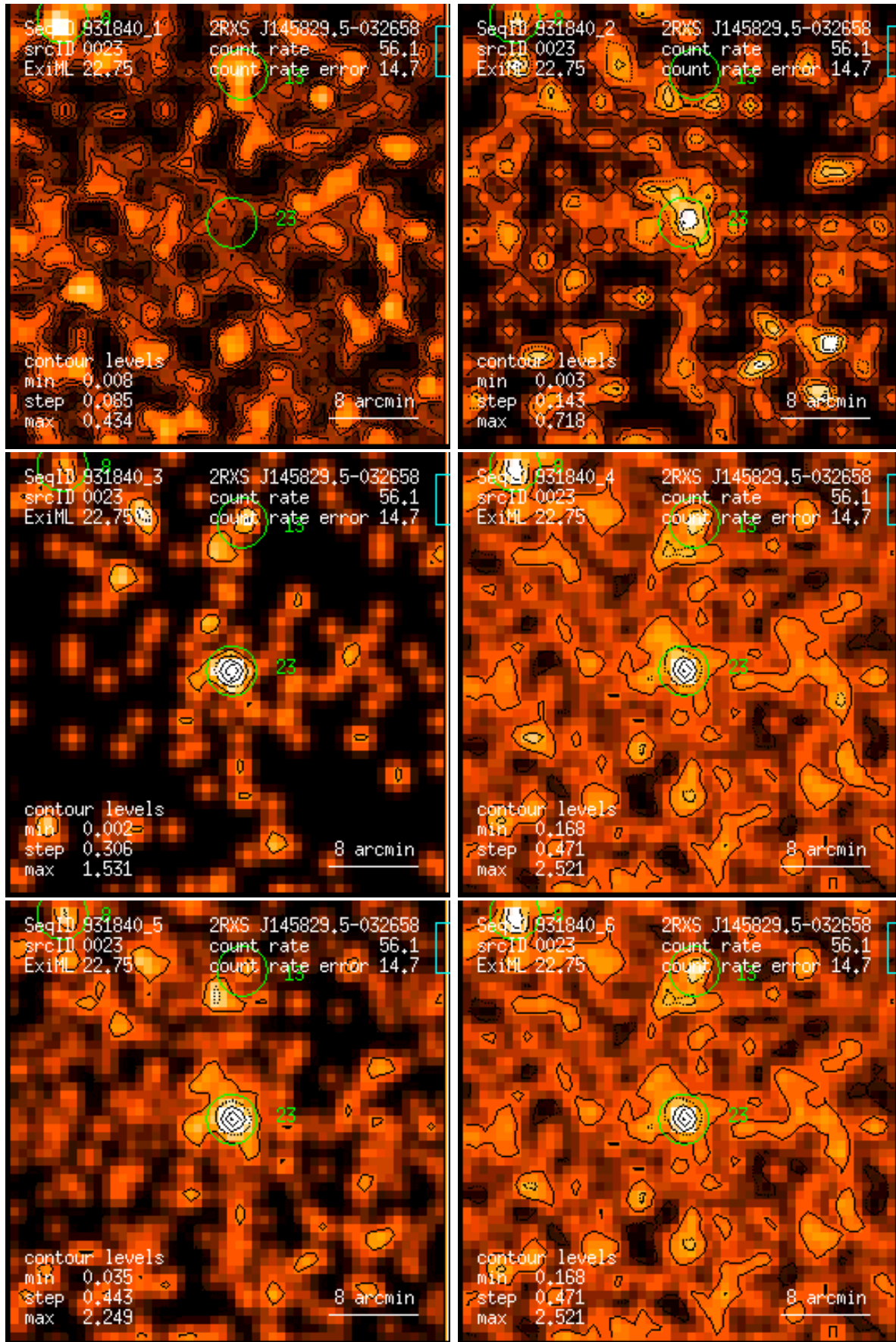
Figure 23: RASS 931840: detection 0023: band rate images, Gaussian filter: (1) PSPC channels 11 – 41, (2) 52 – 90, (3) 91 – 201, (4) 11 – 235, (5) 52 – 201, (6) 11 – 201. Broad band rates in counts/ks. Band rate contour levels in counts/ks/arcmin 2 .
