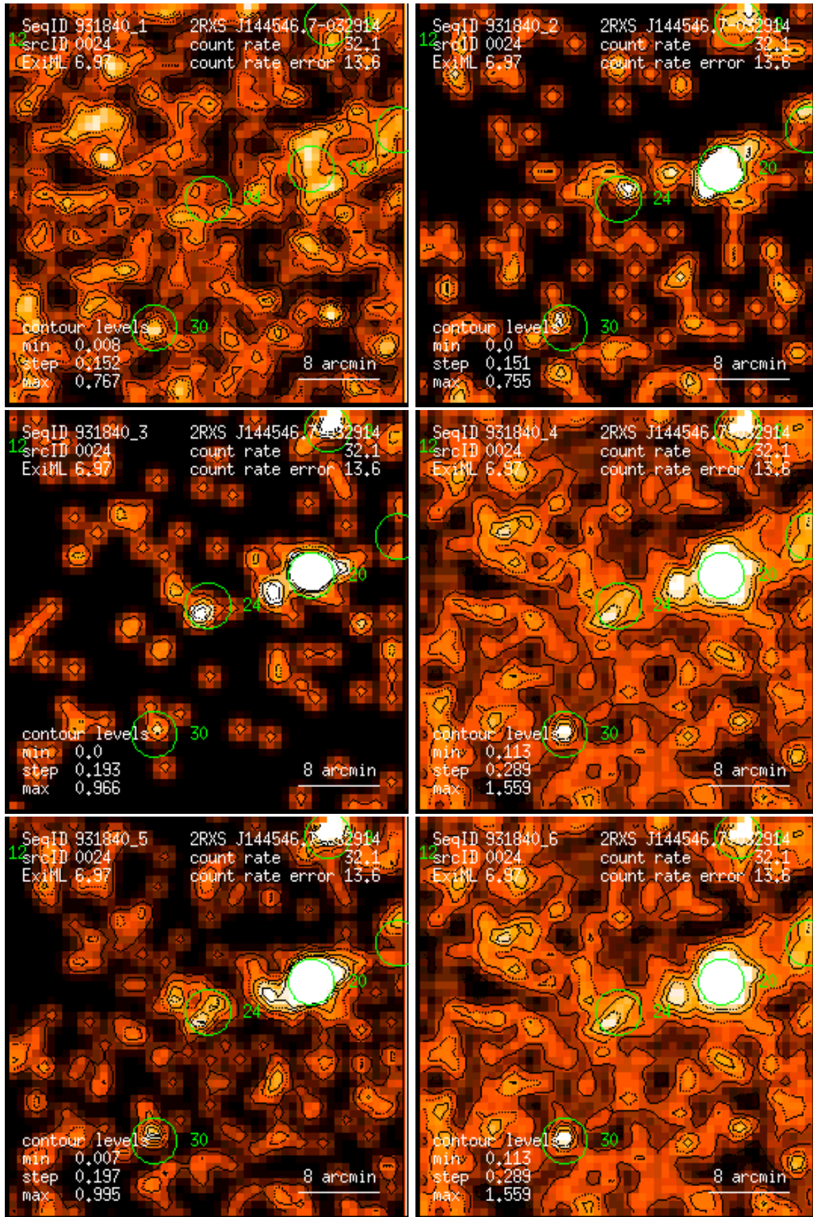
Figure 24: RASS 931840: detection 0024: band rate images, Gaussian filter: (1) PSPC channels 11 – 41, (2) 52 – 90, (3) 91 – 201, (4) 11 – 235, (5) 52 – 201, (6) 11 – 201. Broad band rates in counts/ks. Band rate contour levels in counts/ks/arcmin 2 .
