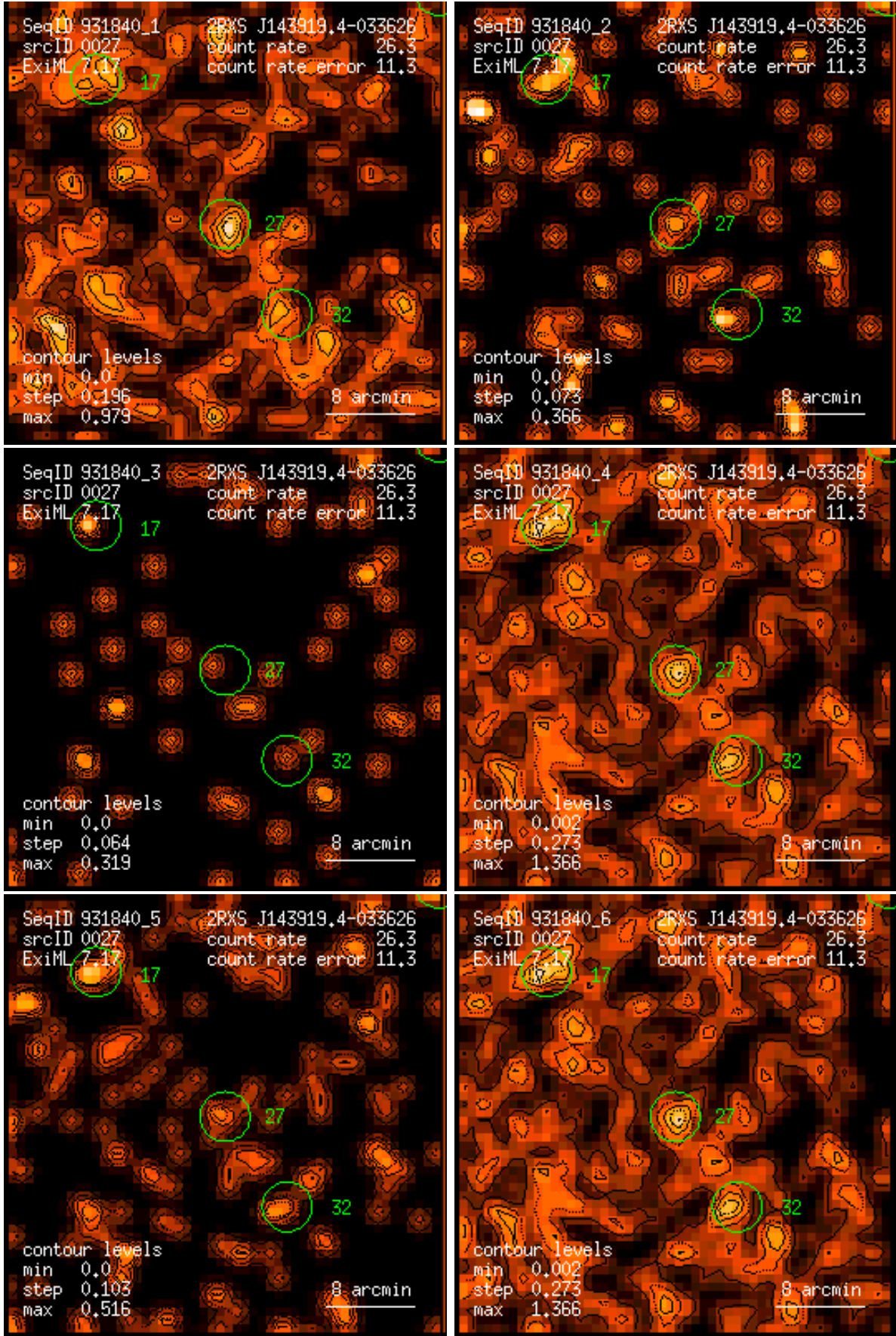
Figure 27: RASS 931840: detection 0027: band rate images, Gaussian filter: (1) PSPC channels 11 – 41, (2) 52 – 90, (3) 91 – 201, (4) 11 – 235, (5) 52 – 201, (6) 11 – 201. Broad band rates in counts/ks. Band rate contour levels in counts/ks/arcmin 2 .
